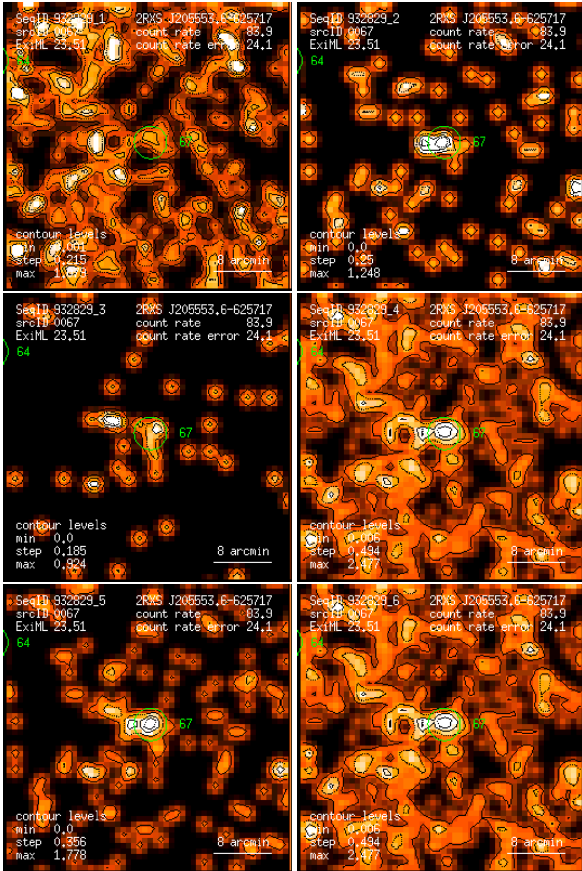
Figure 67: RASS 932829: detection 0067: band rate images, Gaussian filter: (1) PSPC channels 11 – 41, (2) 52 – 90, (3) 91 – 201, (4) 11 – 235, (5) 52 – 201, (6) 11 – 201. Broad band rates in counts/ks. Band rate contour levels in counts/ks/arcmin 2 .
