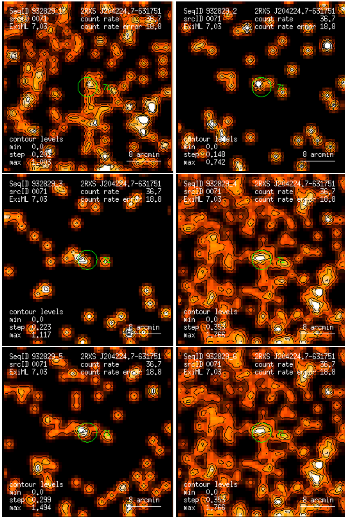
Figure 71: RASS 932829: detection 0071: band rate images, Gaussian filter: (1) PSPC channels 11 – 41, (2) 52 – 90, (3) 91 – 201, (4) 11 – 235, (5) 52 – 201, (6) 11 – 201. Broad band rates in counts/ks. Band rate contour levels in counts/ks/arcmin 2 .
