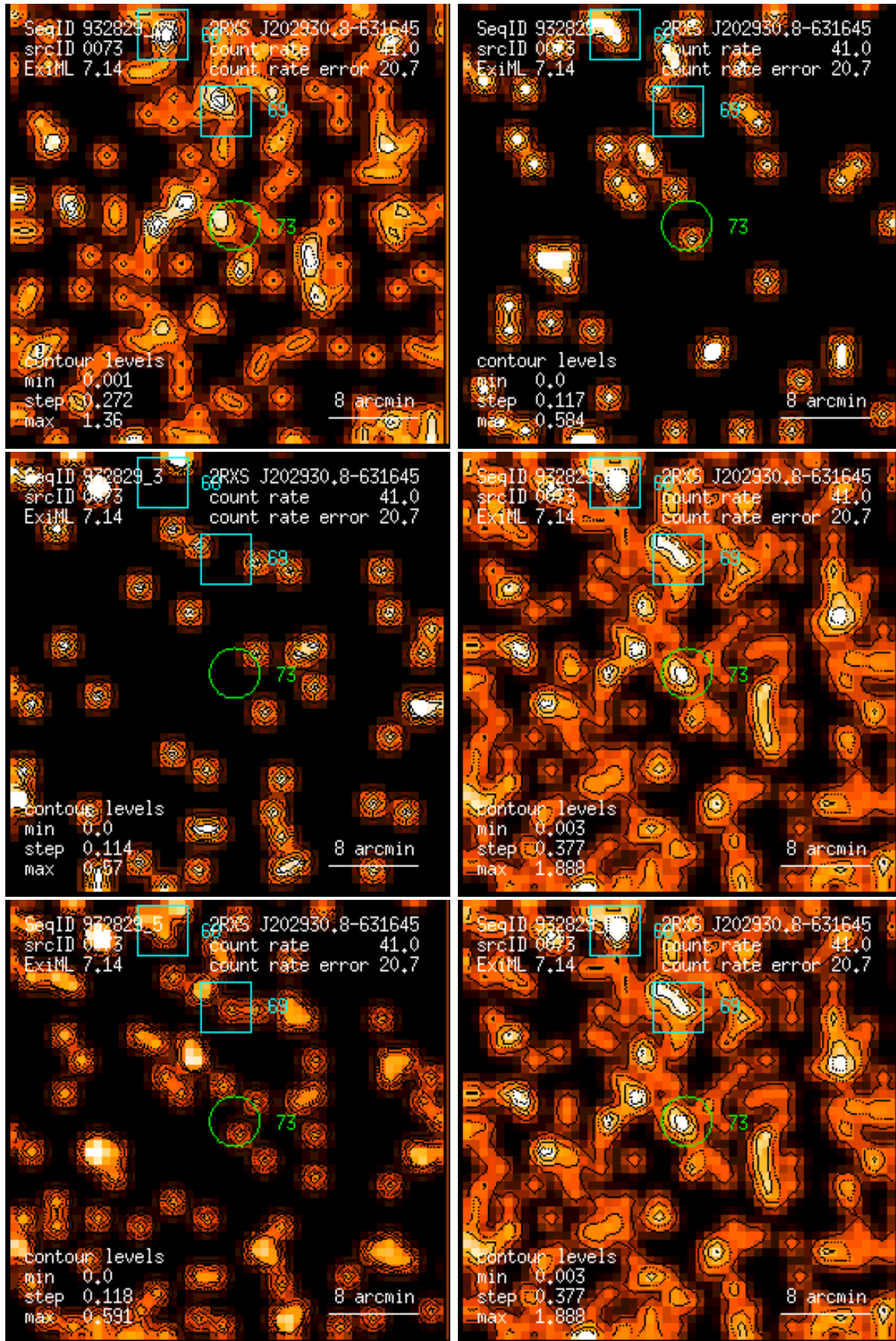
Figure 73: RASS 932829: detection 0073: band rate images, Gaussian filter: (1) PSPC channels 11 – 41, (2) 52 – 90, (3) 91 – 201, (4) 11 – 235, (5) 52 – 201, (6) 11 – 201. Broad band rates in counts/ks. Band rate contour levels in counts/ks/arcmin 2 .
