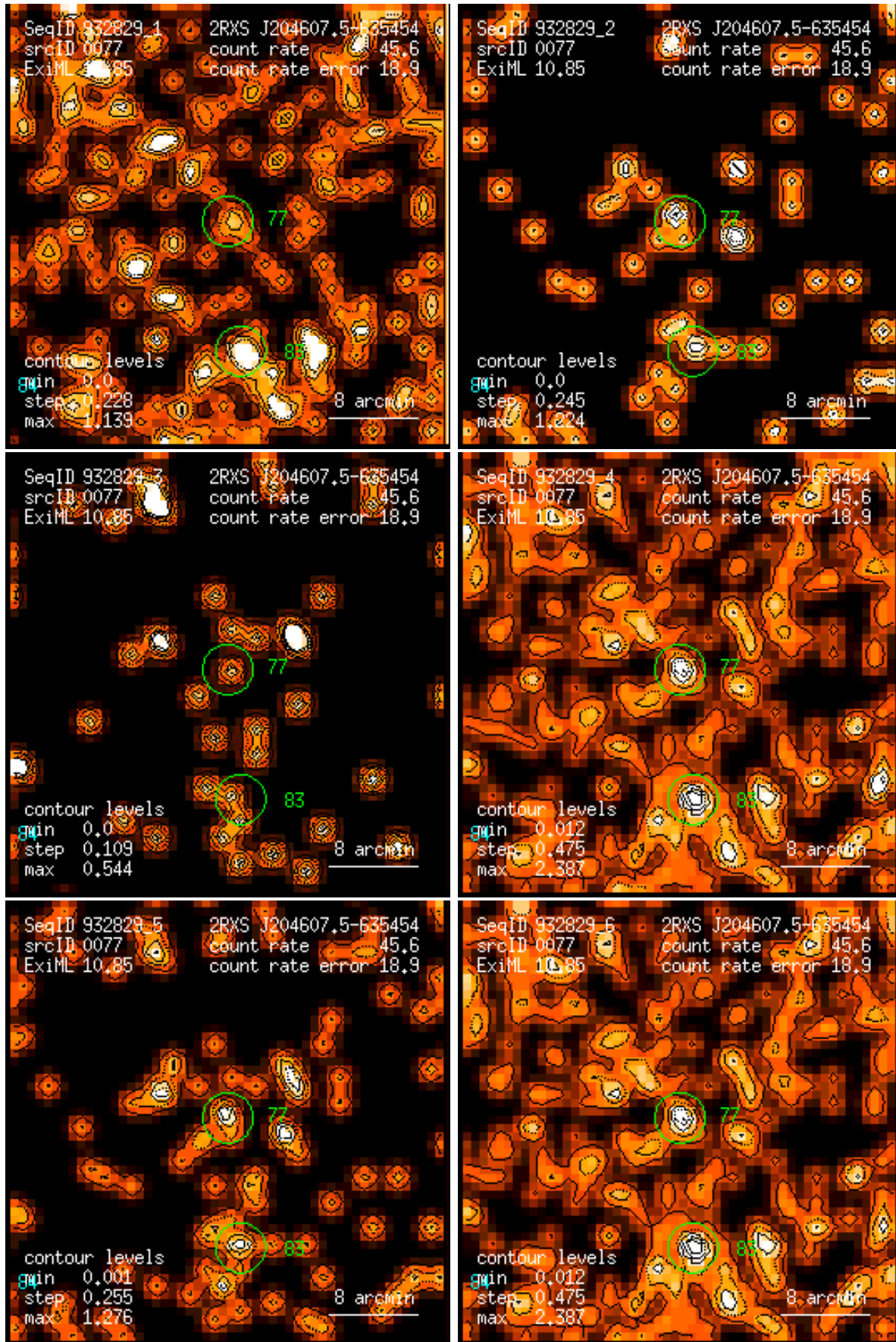
Figure 77: RASS 932829: detection 0077: band rate images, Gaussian filter: (1) PSPC channels 11 – 41, (2) 52 – 90, (3) 91 – 201, (4) 11 – 235, (5) 52 – 201, (6) 11 – 201. Broad band rates in counts/ks. Band rate contour levels in counts/ks/arcmin 2 .
