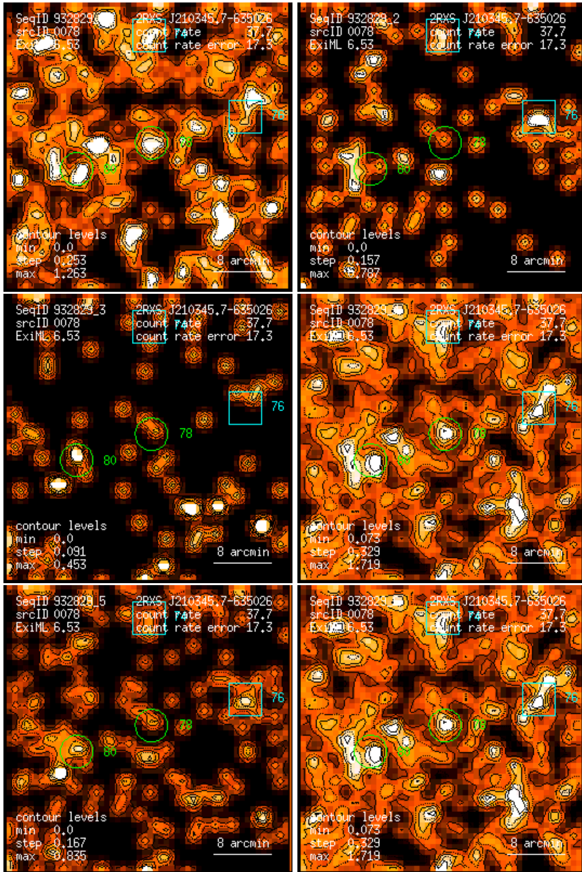
Figure 78: RASS 932829: detection 0078: band rate images, Gaussian filter: (1) PSPC channels 11 – 41, (2) 52 – 90, (3) 91 – 201, (4) 11 – 235, (5) 52 – 201, (6) 11 – 201. Broad band rates in counts/ks. Band rate contour levels in counts/ks/arcmin 2 .
