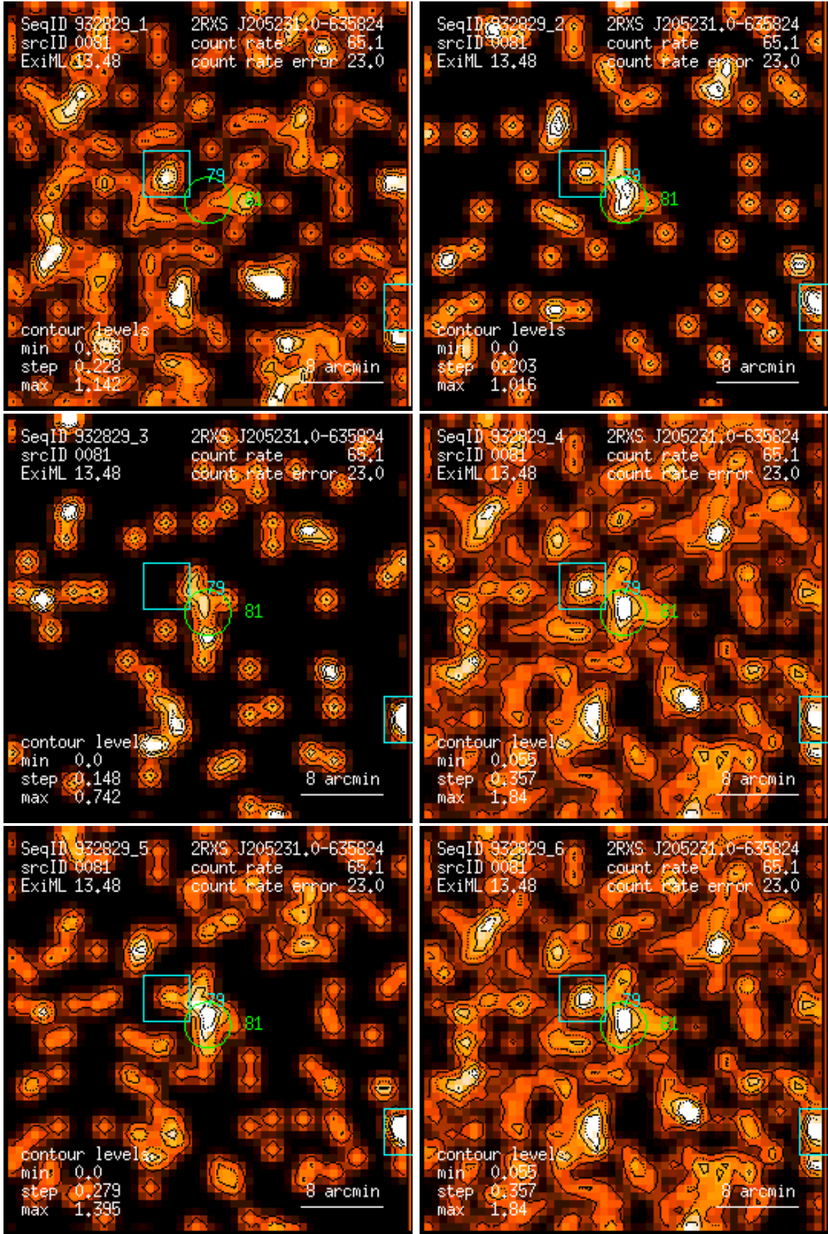
Figure 81: RASS 932829: detection 0081: band rate images, Gaussian filter: (1) PSPC channels 11 – 41, (2) 52 – 90, (3) 91 – 201, (4) 11 – 235, (5) 52 – 201, (6) 11 – 201. Broad band rates in counts/ks. Band rate contour levels in counts/ks/arcmin 2 .
