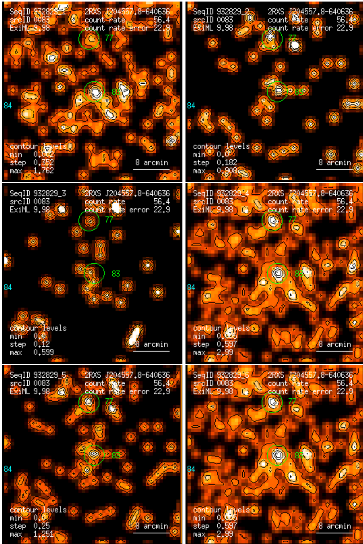
Figure 83: RASS 932829: detection 0083: band rate images, Gaussian filter: (1) PSPC channels 11 – 41, (2) 52 – 90, (3) 91 – 201, (4) 11 – 235, (5) 52 – 201, (6) 11 – 201. Broad band rates in counts/ks. Band rate contour levels in counts/ks/arcmin 2 .
