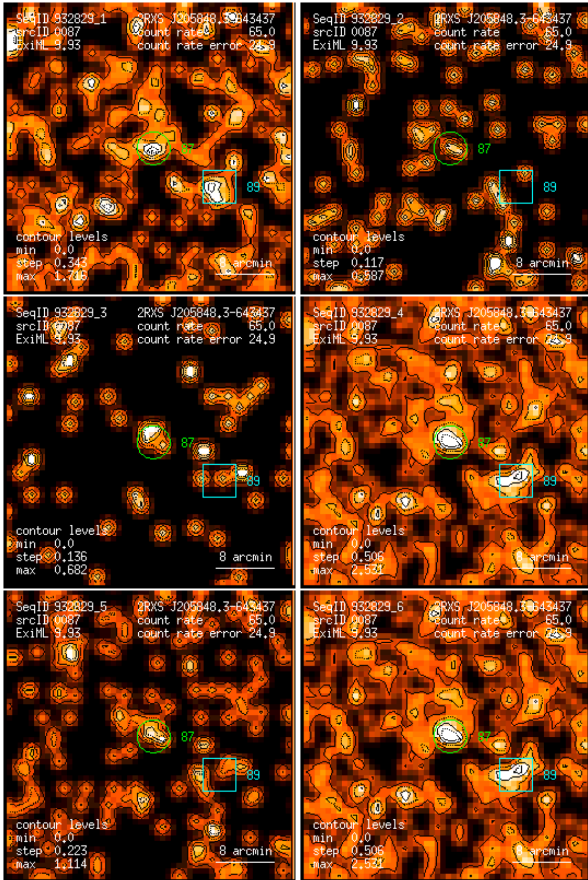
Figure 87: RASS 932829: detection 0087: band rate images, Gaussian filter: (1) PSPC channels 11 – 41, (2) 52 – 90, (3) 91 – 201, (4) 11 – 235, (5) 52 – 201, (6) 11 – 201. Broad band rates in counts/ks. Band rate contour levels in counts/ks/arcmin 2 .
