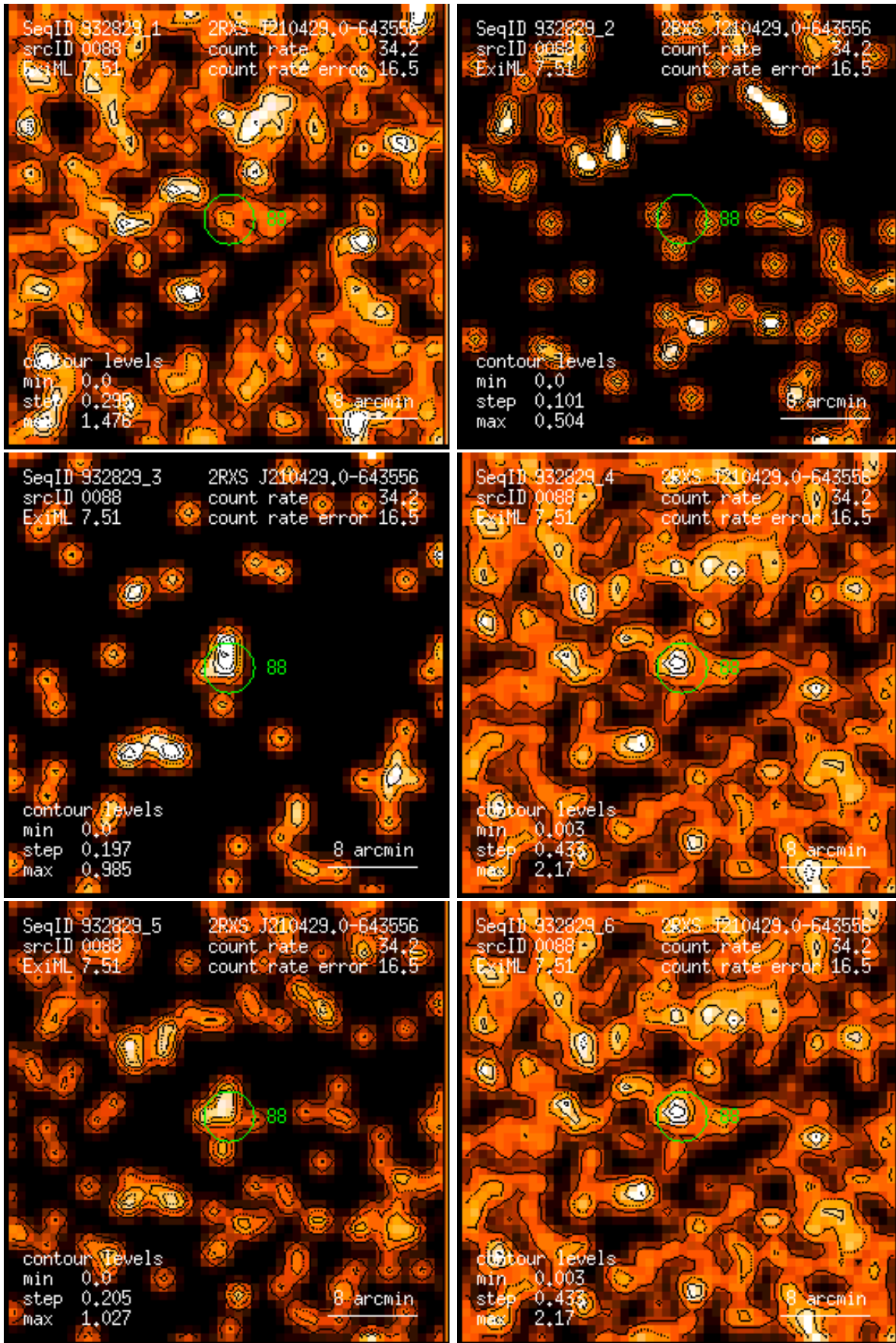
Figure 88: RASS 932829: detection 0088: band rate images, Gaussian filter: (1) PSPC channels 11 – 41, (2) 52 – 90, (3) 91 – 201, (4) 11 – 235, (5) 52 – 201, (6) 11 – 201. Broad band rates in counts/ks. Band rate contour levels in counts/ks/arcmin 2 .
