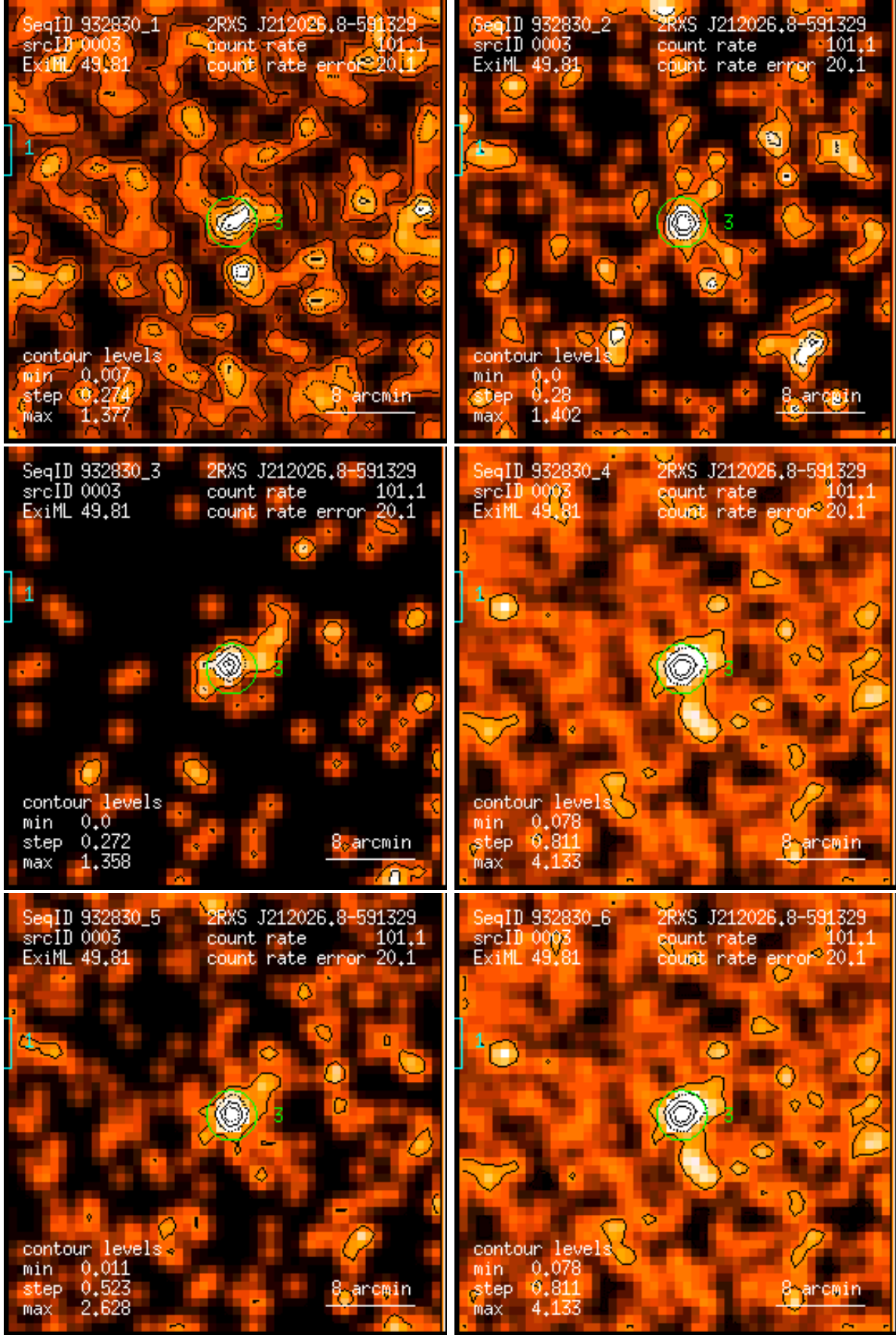
Figure 3: RASS 932830: detection 0003: band rate images, Gaussian filter: (1) PSPC channels 11 – 41, (2) 52 – 90, (3) 91 – 201, (4) 11 – 235, (5) 52 – 201, (6) 11 – 201. Broad band rates in counts/ks. Band rate contour levels in counts/ks/arcmin 2 .
