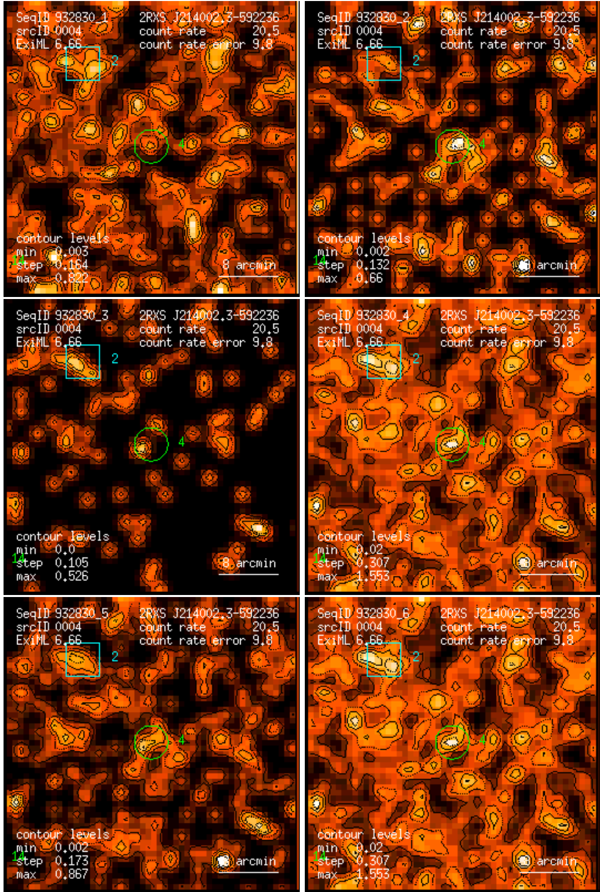
Figure 4: RASS 932830: detection 0004: band rate images, Gaussian filter: (1) PSPC channels 11 – 41, (2) 52 – 90, (3) 91 – 201, (4) 11 – 235, (5) 52 – 201, (6) 11 – 201. Broad band rates in counts/ks. Band rate contour levels in counts/ks/arcmin 2 .
