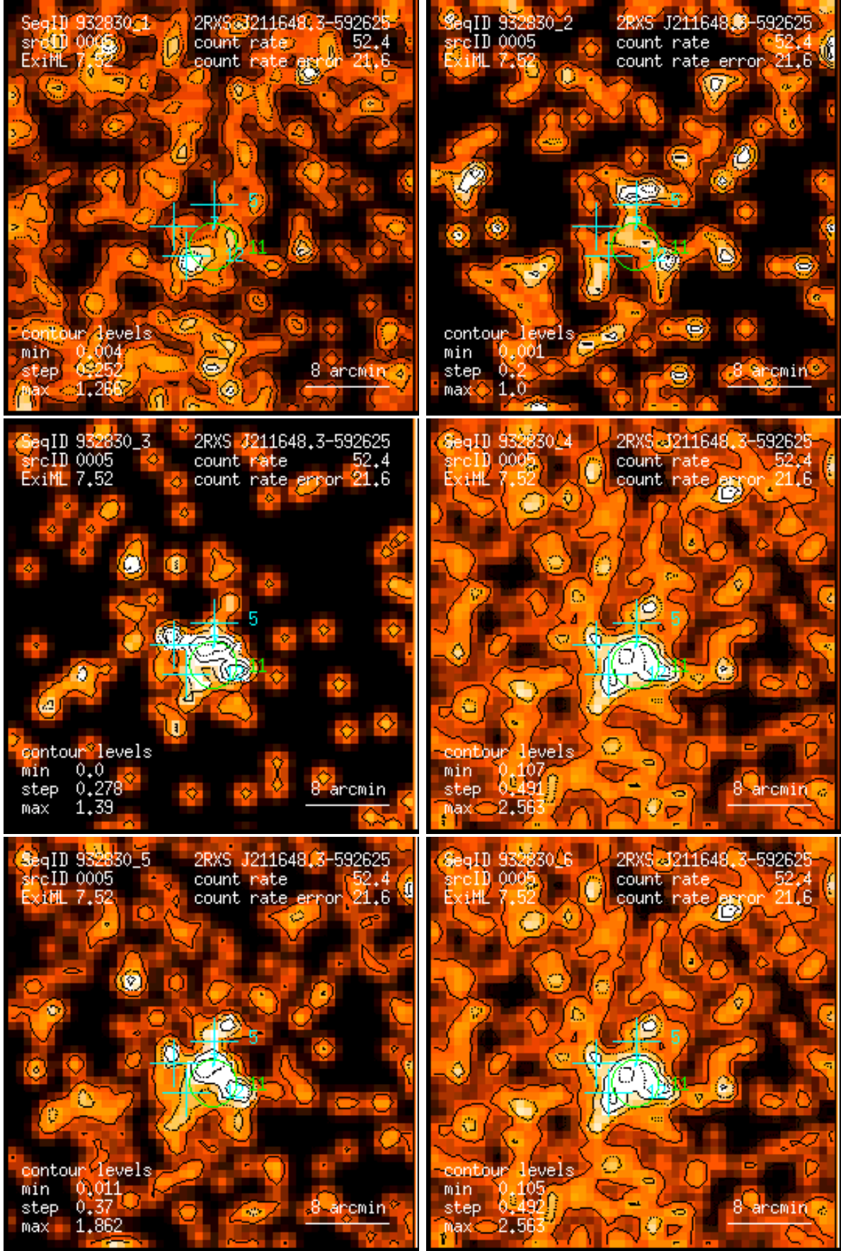
Figure 5: RASS 932830: detection 0005: band rate images, Gaussian filter: (1) PSPC channels 11 – 41, (2) 52 – 90, (3) 91 – 201, (4) 11 – 235, (5) 52 – 201, (6) 11 – 201. Broad band rates in counts/ks. Band rate contour levels in counts/ks/arcmin 2 .
