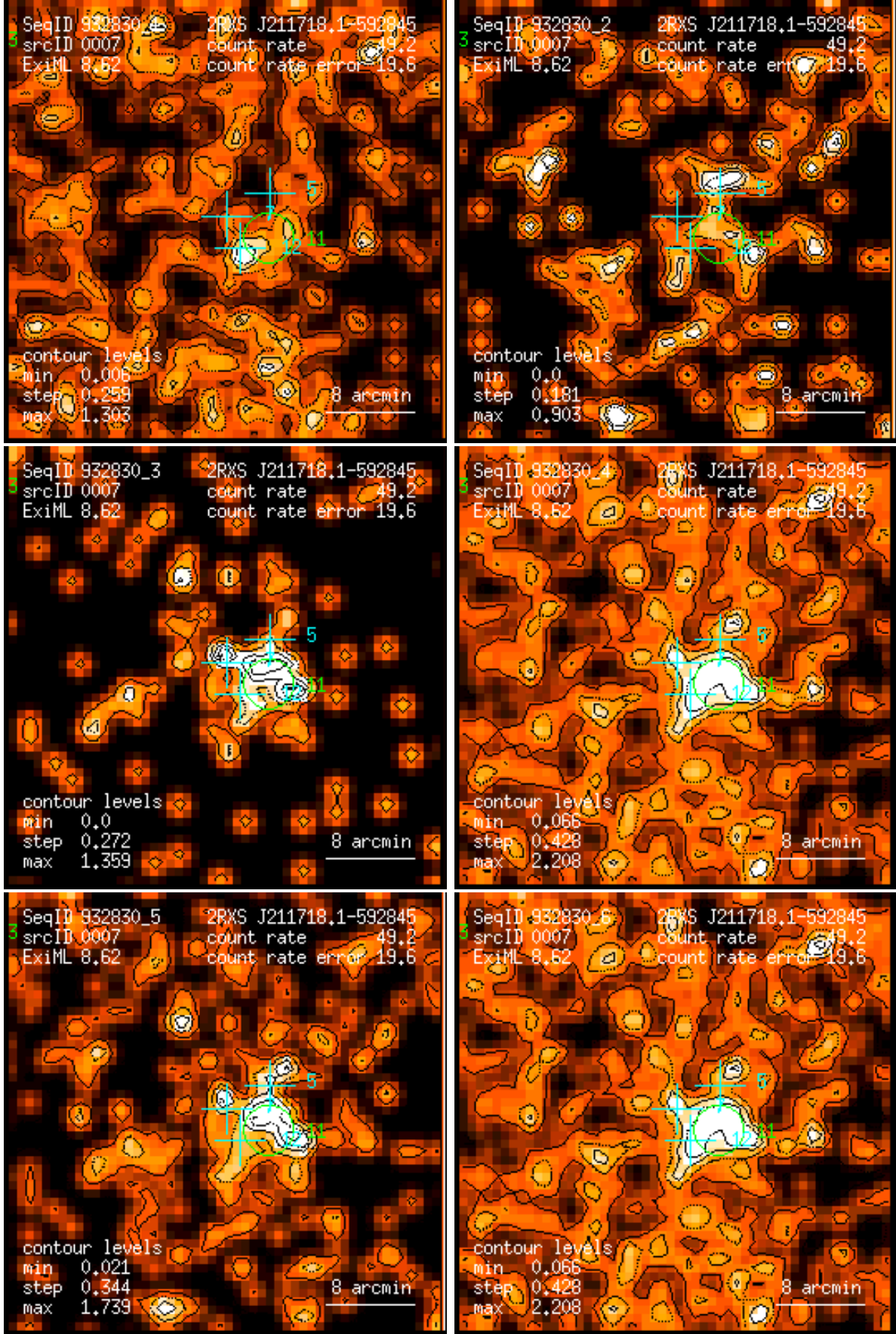
Figure 7: RASS 932830: detection 0007: band rate images, Gaussian filter: (1) PSPC channels 11 – 41, (2) 52 – 90, (3) 91 – 201, (4) 11 – 235, (5) 52 – 201, (6) 11 – 201. Broad band rates in counts/ks. Band rate contour levels in counts/ks/arcmin 2 .
