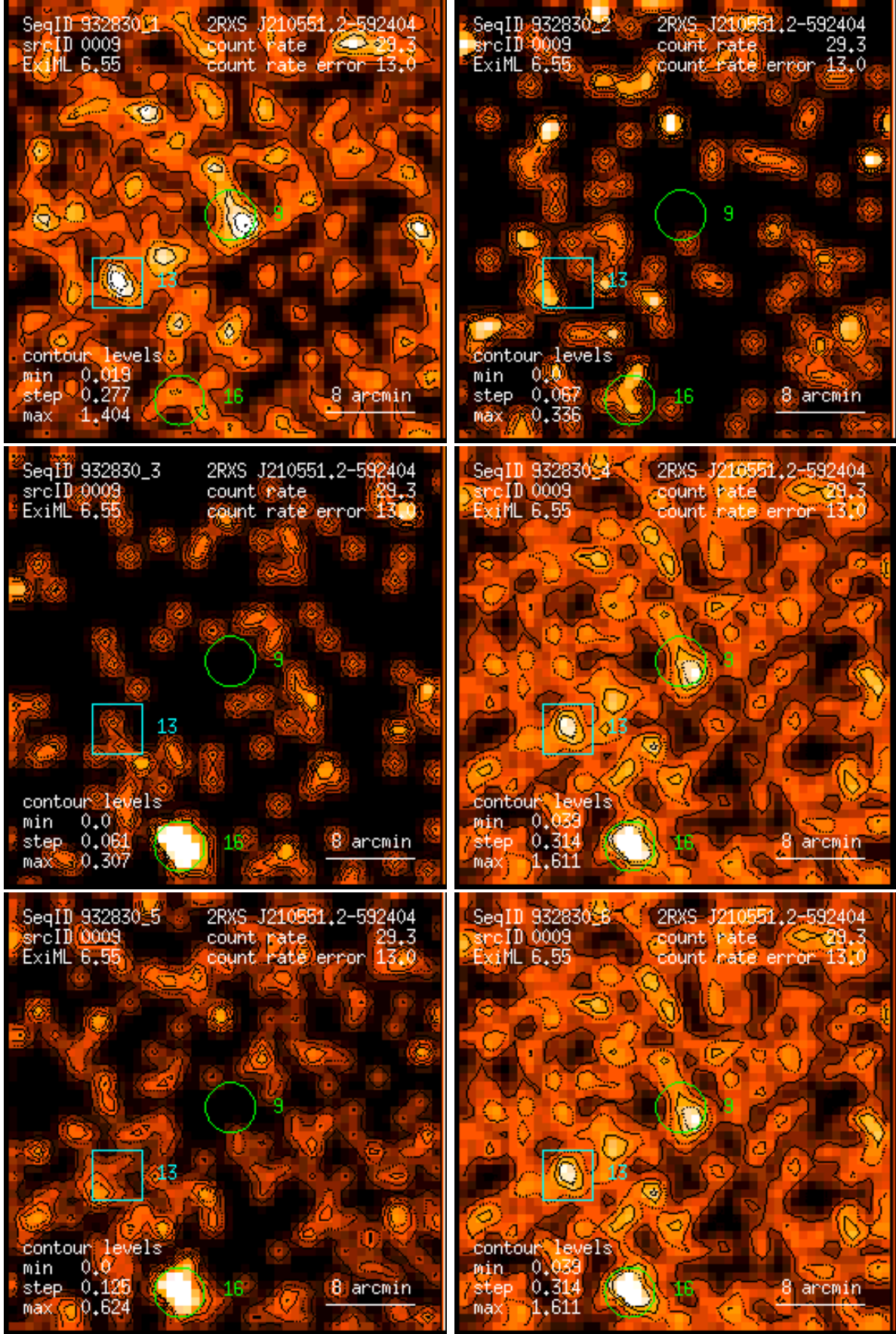
Figure 9: RASS 932830: detection 0009: band rate images, Gaussian filter: (1) PSPC channels 11 – 41, (2) 52 – 90, (3) 91 – 201, (4) 11 – 235, (5) 52 – 201, (6) 11 – 201. Broad band rates in counts/ks. Band rate contour levels in counts/ks/arcmin 2 .
