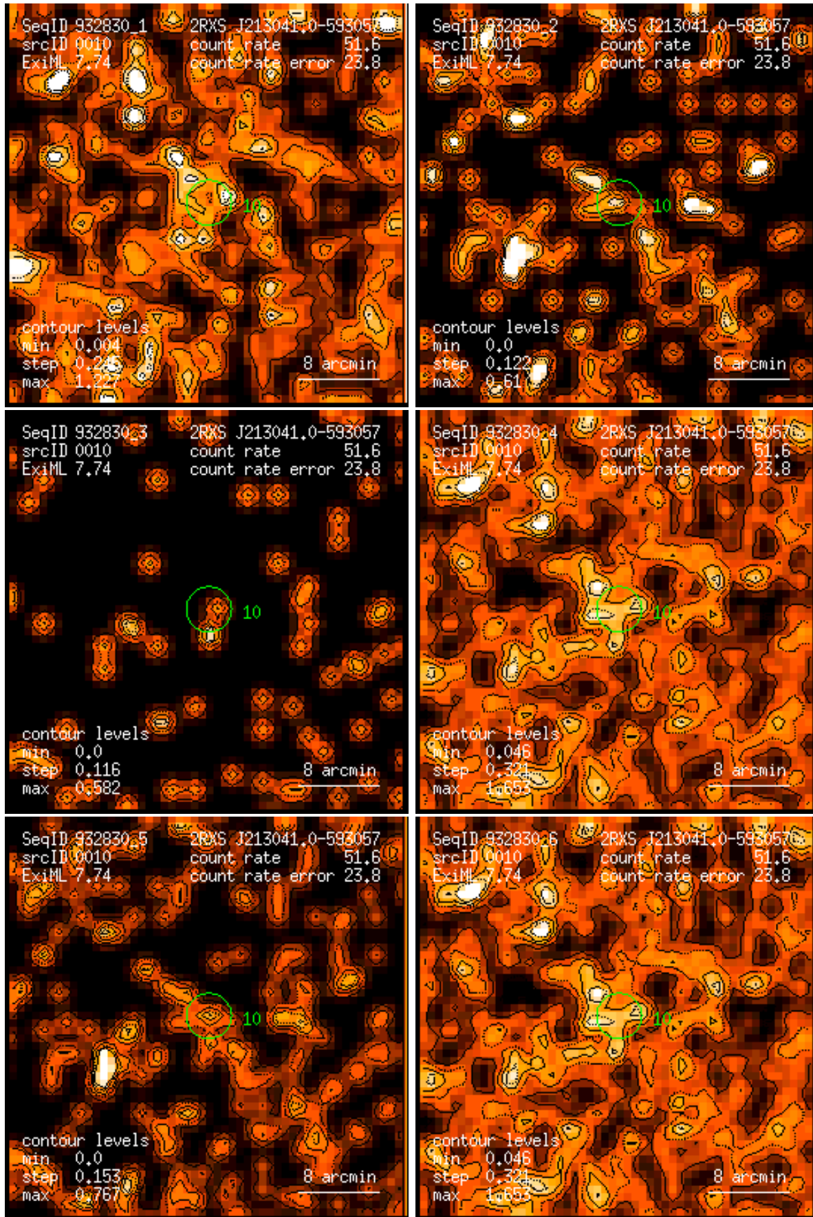
Figure 10: RASS 932830: detection 0010: band rate images, Gaussian filter: (1) PSPC channels 11 – 41, (2) 52 – 90, (3) 91 – 201, (4) 11 – 235, (5) 52 – 201, (6) 11 – 201. Broad band rates in counts/ks. Band rate contour levels in counts/ks/arcmin 2 .
