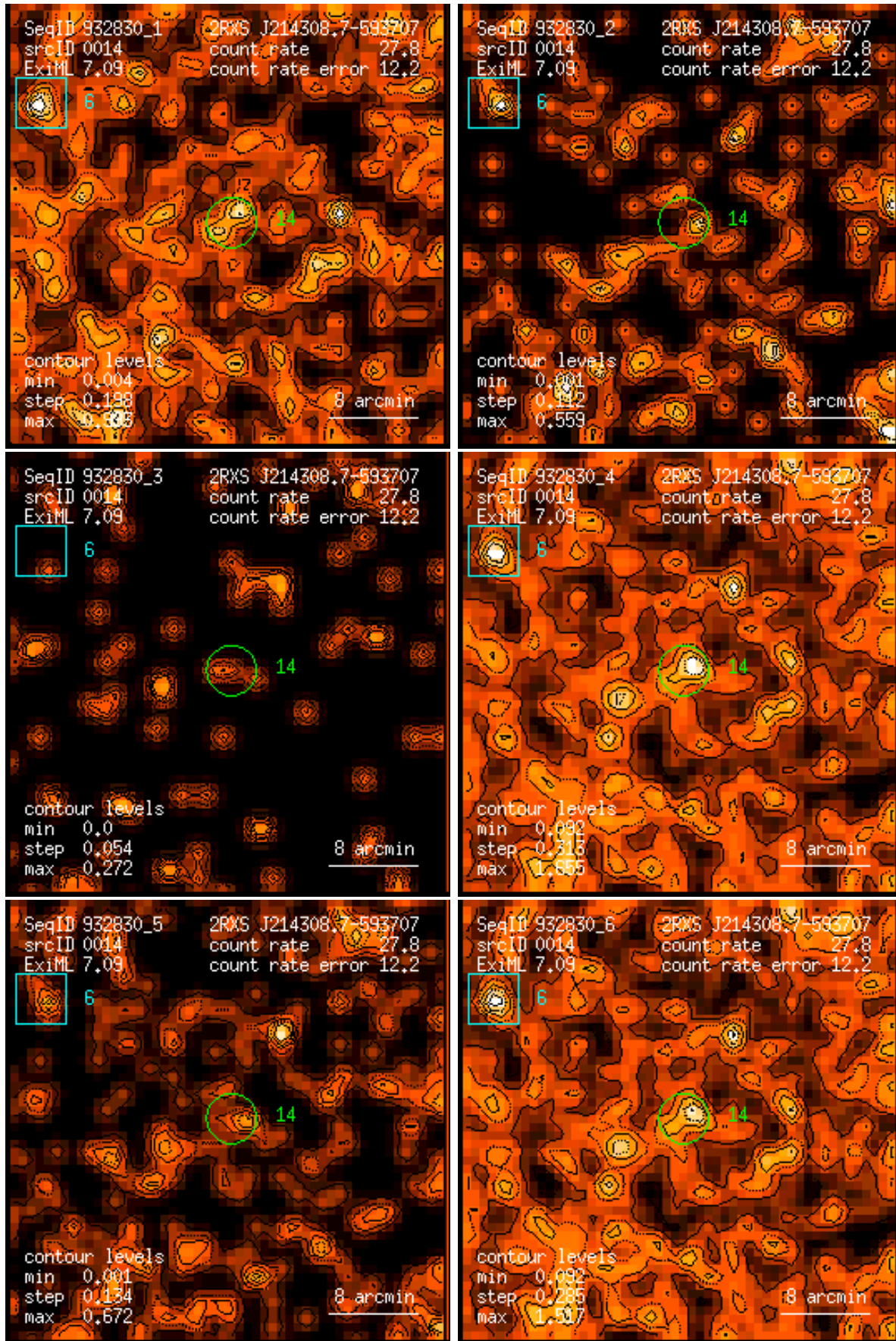
Figure 14: RASS 932830: detection 0014: band rate images, Gaussian filter: (1) PSPC channels 11 – 41, (2) 52 – 90, (3) 91 – 201, (4) 11 – 235, (5) 52 – 201, (6) 11 – 201. Broad band rates in counts/ks. Band rate contour levels in counts/ks/arcmin 2 .
