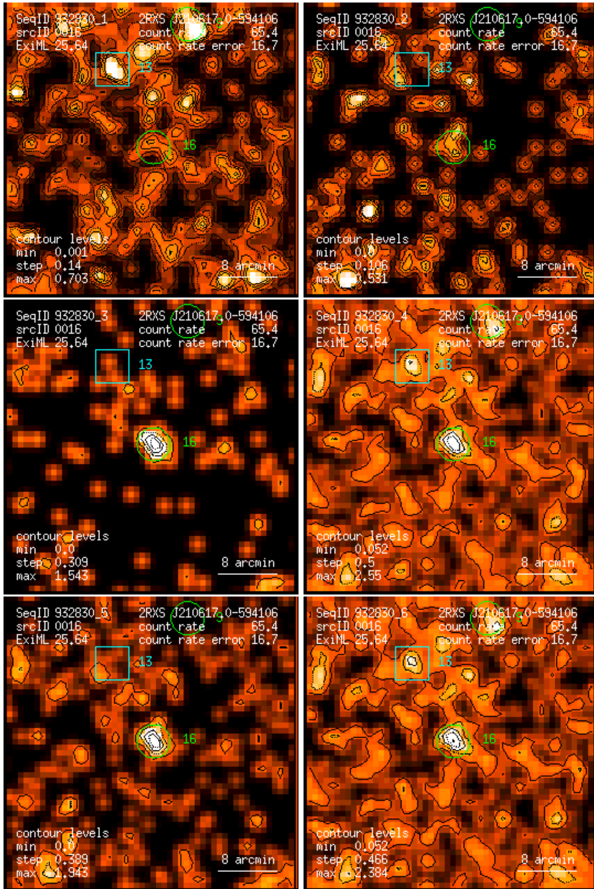
Figure 16: RASS 932830: detection 0016: band rate images, Gaussian filter: (1) PSPC channels 11 – 41, (2) 52 – 90, (3) 91 – 201, (4) 11 – 235, (5) 52 – 201, (6) 11 – 201. Broad band rates in counts/ks. Band rate contour levels in counts/ks/arcmin 2 .
