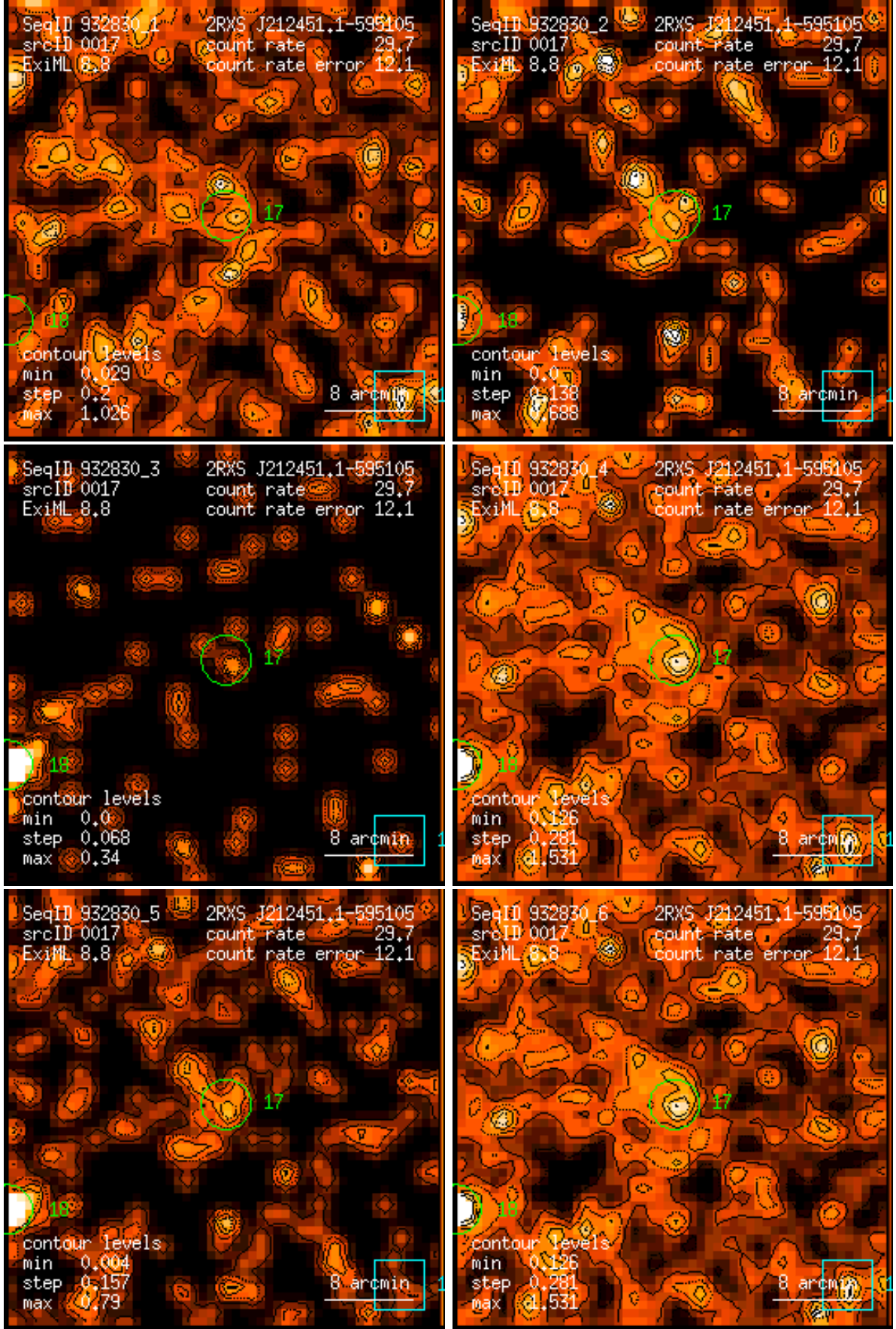
Figure 17: RASS 932830: detection 0017: band rate images, Gaussian filter: (1) PSPC channels 11 – 41, (2) 52 – 90, (3) 91 – 201, (4) 11 – 235, (5) 52 – 201, (6) 11 – 201. Broad band rates in counts/ks. Band rate contour levels in counts/ks/arcmin 2 .
