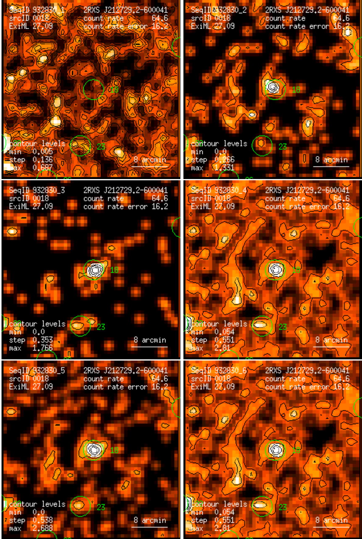
Figure 18: RASS 932830: detection 0018: band rate images, Gaussian filter: (1) PSPC channels 11 – 41, (2) 52 – 90, (3) 91 – 201, (4) 11 – 235, (5) 52 – 201, (6) 11 – 201. Broad band rates in counts/ks. Band rate contour levels in counts/ks/arcmin 2 .
