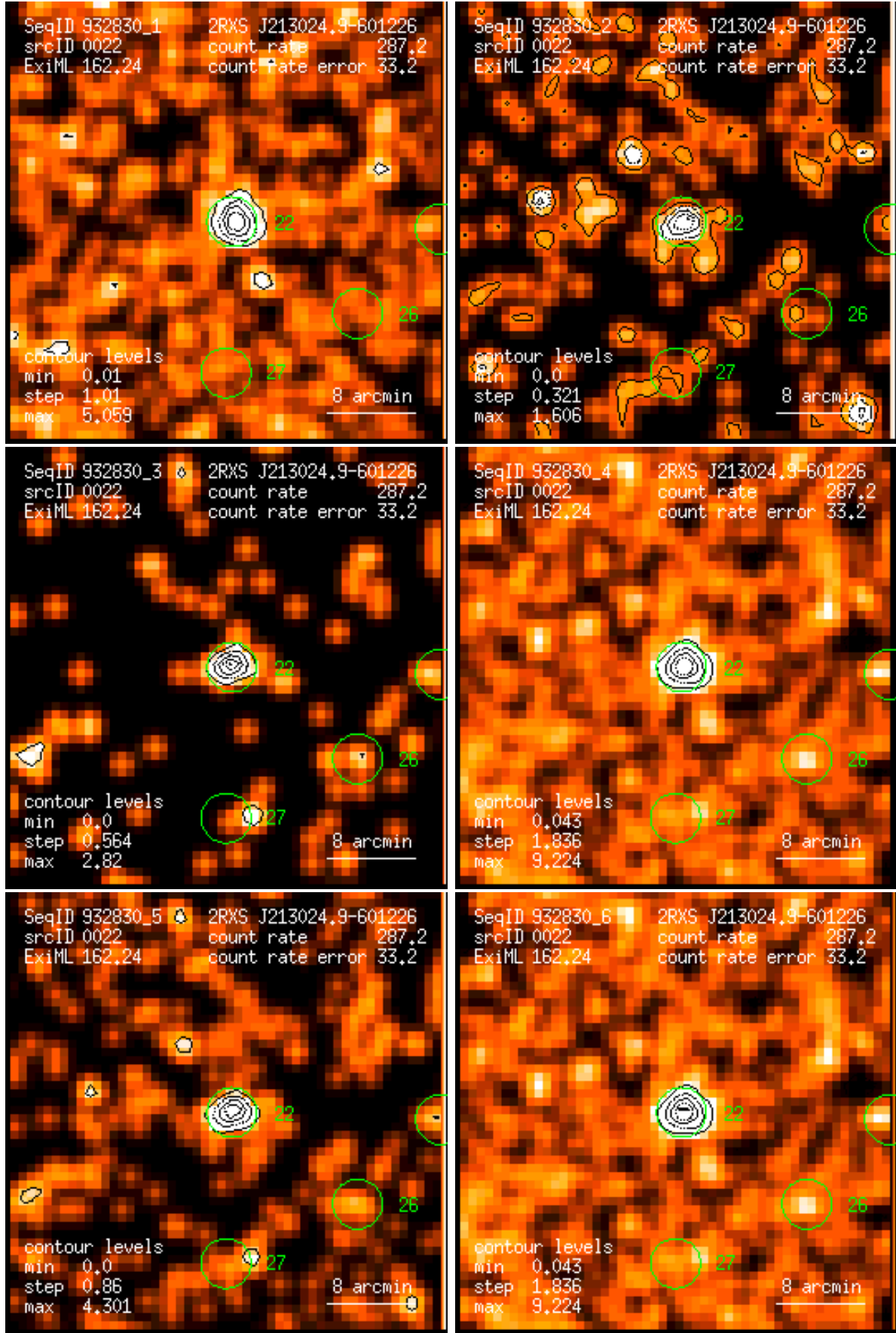
Figure 22: RASS 932830: detection 0022: band rate images, Gaussian filter: (1) PSPC channels 11 – 41, (2) 52 – 90, (3) 91 – 201, (4) 11 – 235, (5) 52 – 201, (6) 11 – 201. Broad band rates in counts/ks. Band rate contour levels in counts/ks/arcmin 2 .
