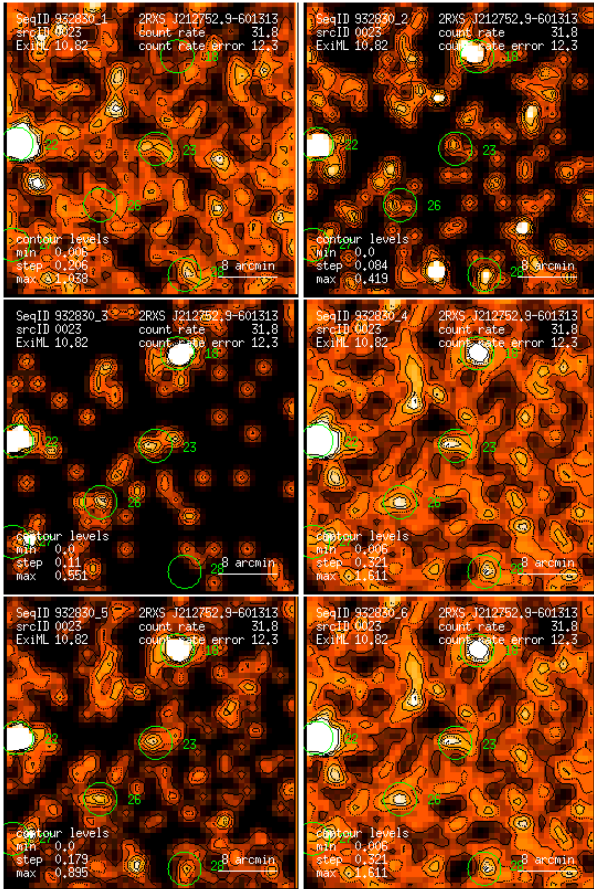
Figure 23: RASS 932830: detection 0023: band rate images, Gaussian filter: (1) PSPC channels 11 – 41, (2) 52 – 90, (3) 91 – 201, (4) 11 – 235, (5) 52 – 201, (6) 11 – 201. Broad band rates in counts/ks. Band rate contour levels in counts/ks/arcmin 2 .
