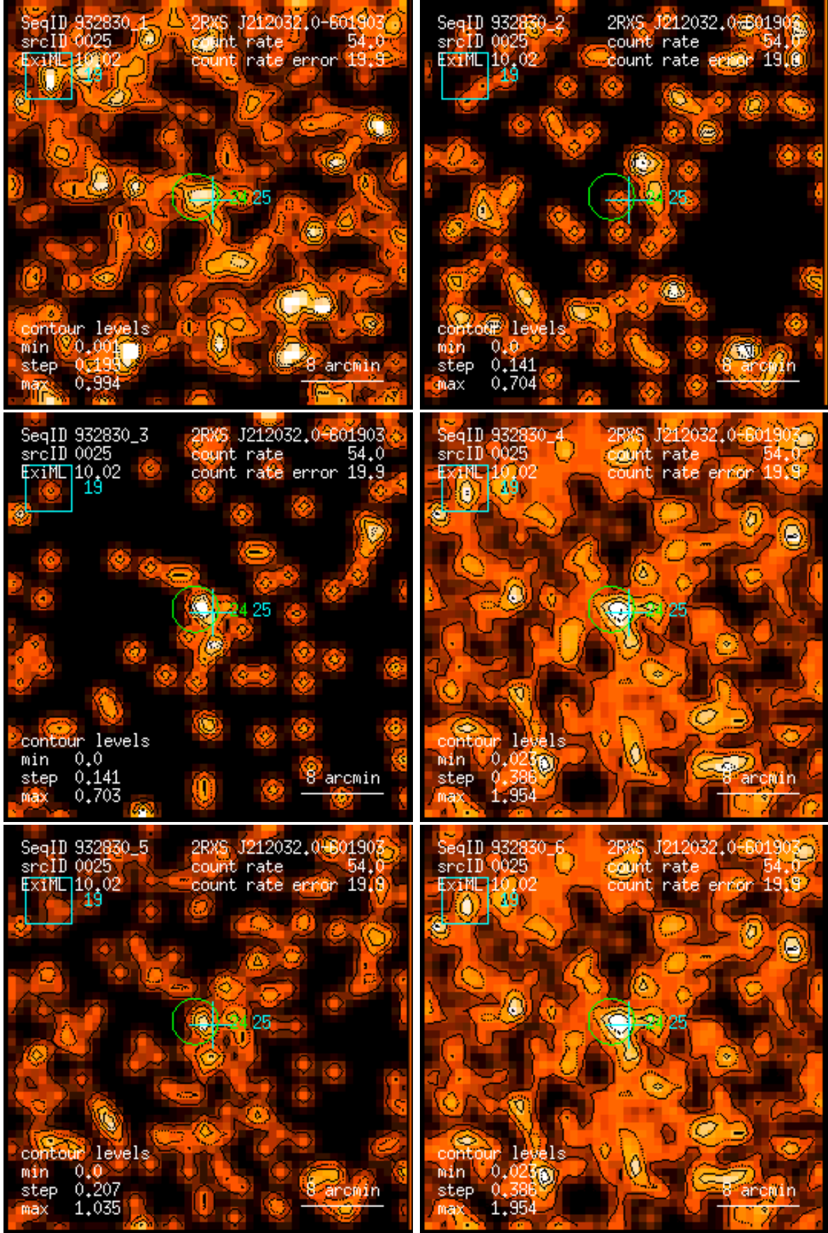
Figure 25: RASS 932830: detection 0025: band rate images, Gaussian filter: (1) PSPC channels 11 – 41, (2) 52 – 90, (3) 91 – 201, (4) 11 – 235, (5) 52 – 201, (6) 11 – 201. Broad band rates in counts/ks. Band rate contour levels in counts/ks/arcmin 2 .
