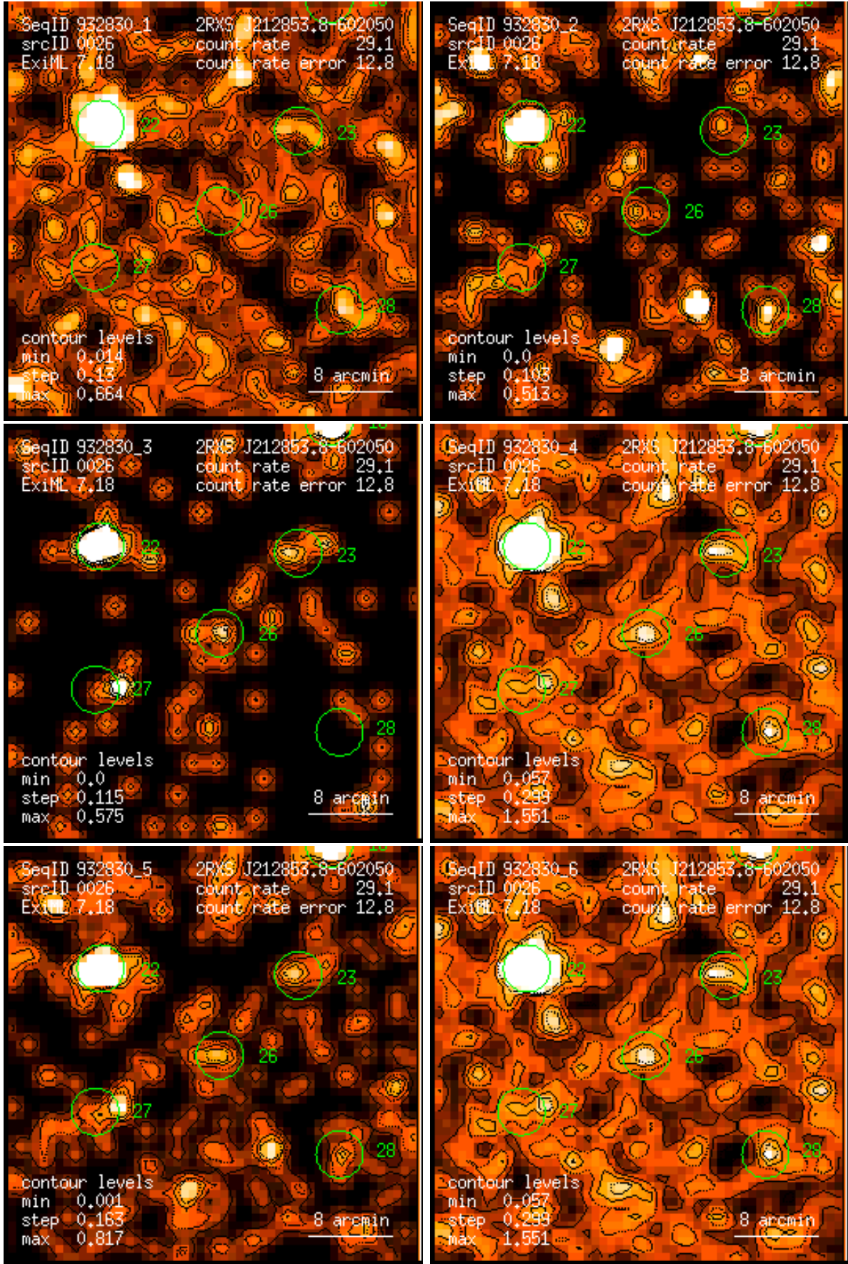
Figure 26: RASS 932830: detection 0026: band rate images, Gaussian filter: (1) PSPC channels 11 – 41, (2) 52 – 90, (3) 91 – 201, (4) 11 – 235, (5) 52 – 201, (6) 11 – 201. Broad band rates in counts/ks. Band rate contour levels in counts/ks/arcmin 2 .
