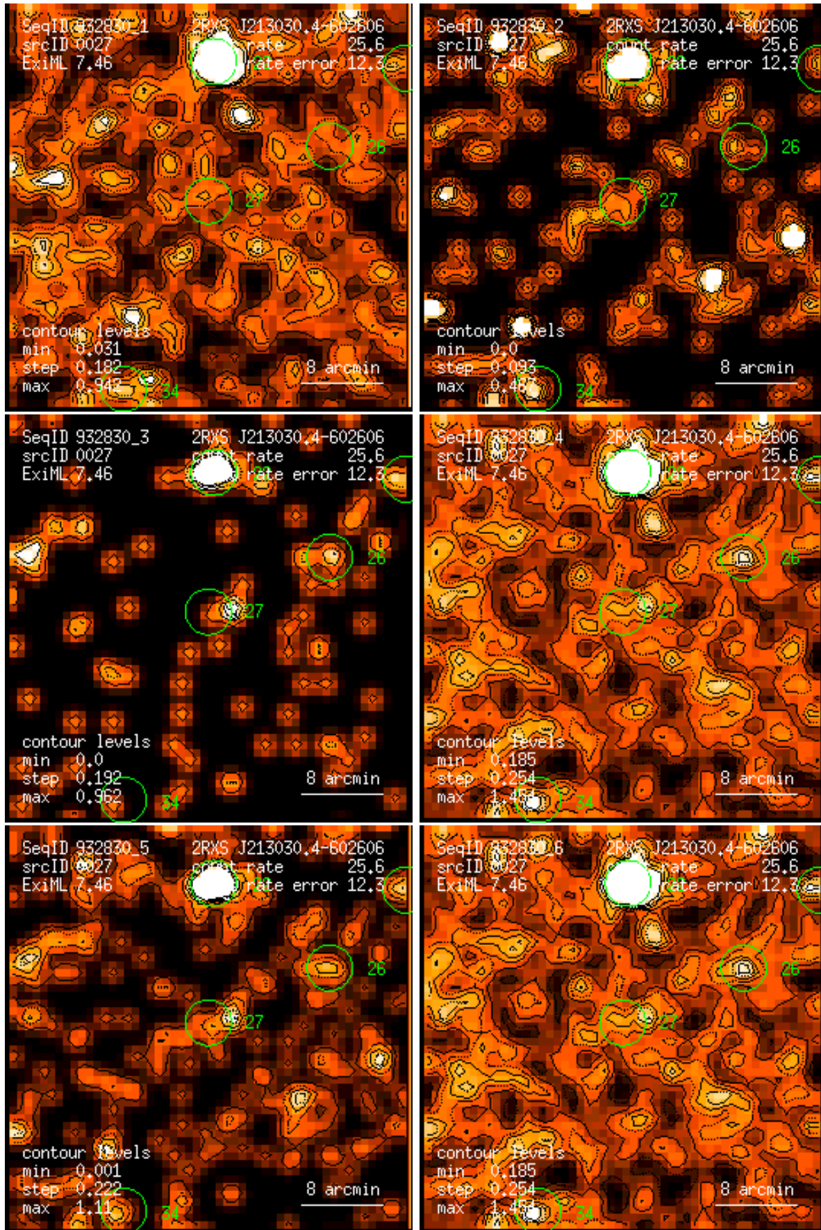
Figure 27: RASS 932830: detection 0027: band rate images, Gaussian filter: (1) PSPC channels 11 – 41, (2) 52 – 90, (3) 91 – 201, (4) 11 – 235, (5) 52 – 201, (6) 11 – 201. Broad band rates in counts/ks. Band rate contour levels in counts/ks/arcmin 2 .
