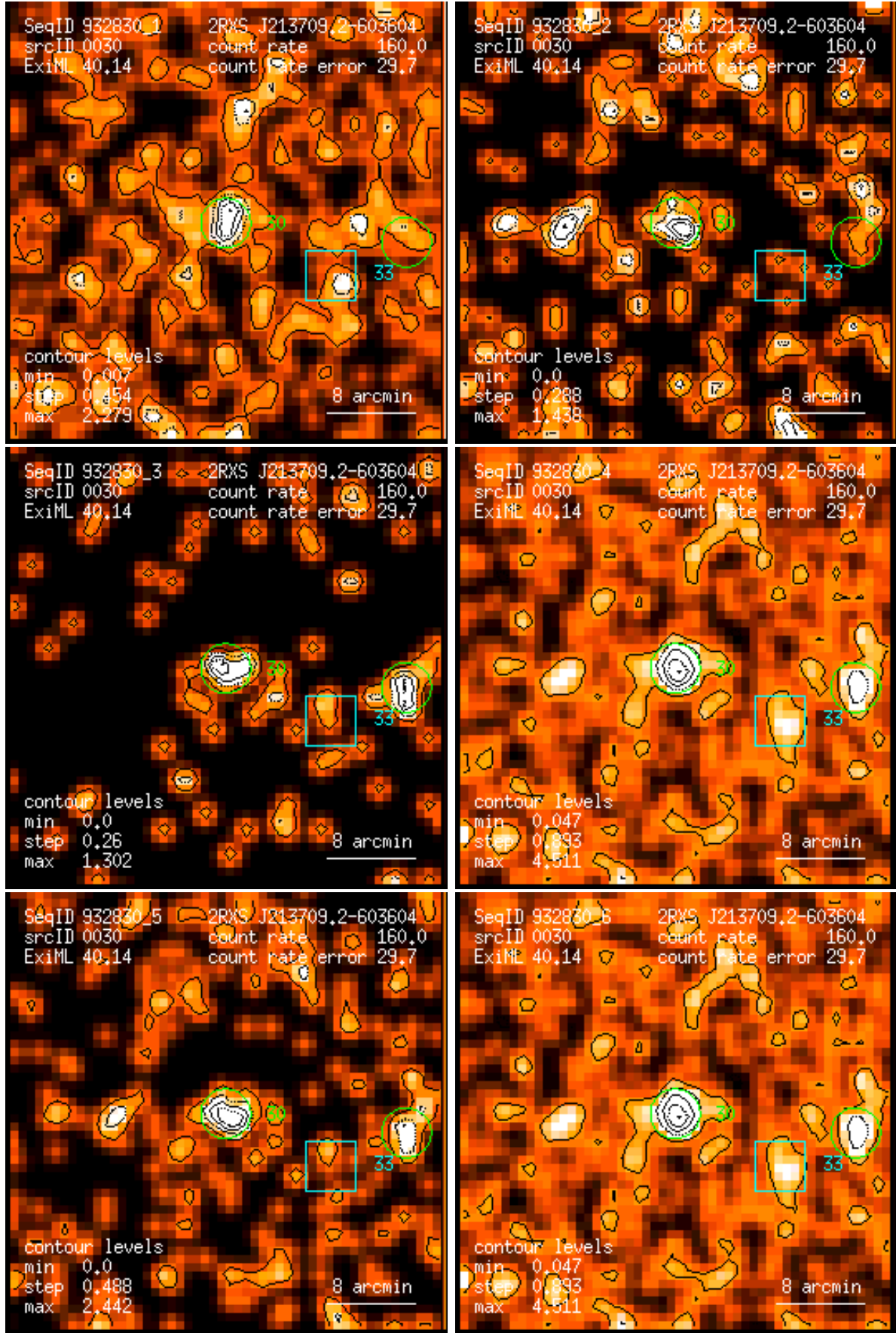
Figure 30: RASS 932830: detection 0030: band rate images, Gaussian filter: (1) PSPC channels 11 – 41, (2) 52 – 90, (3) 91 – 201, (4) 11 – 235, (5) 52 – 201, (6) 11 – 201. Broad band rates in counts/ks. Band rate contour levels in counts/ks/arcmin 2 .
