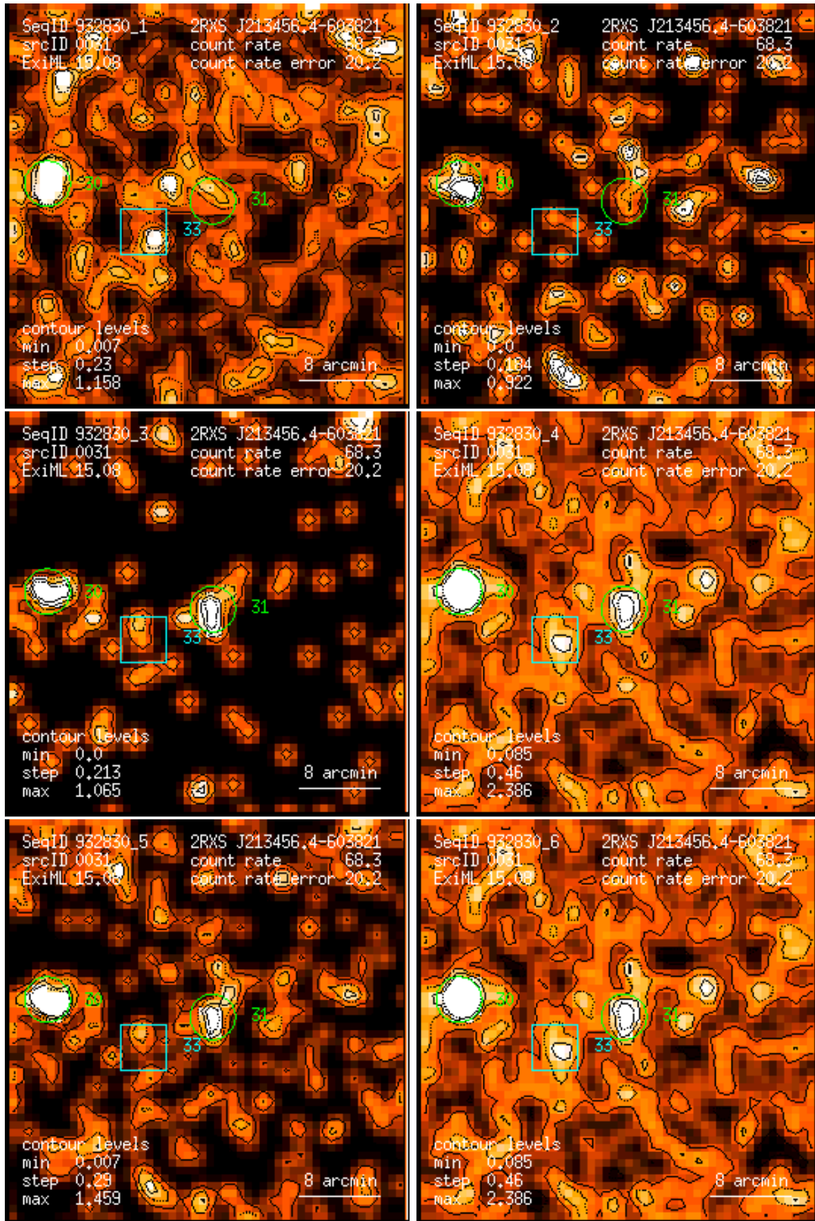
Figure 31: RASS 932830: detection 0031: band rate images, Gaussian filter: (1) PSPC channels 11 – 41, (2) 52 – 90, (3) 91 – 201, (4) 11 – 235, (5) 52 – 201, (6) 11 – 201. Broad band rates in counts/ks. Band rate contour levels in counts/ks/arcmin 2 .
