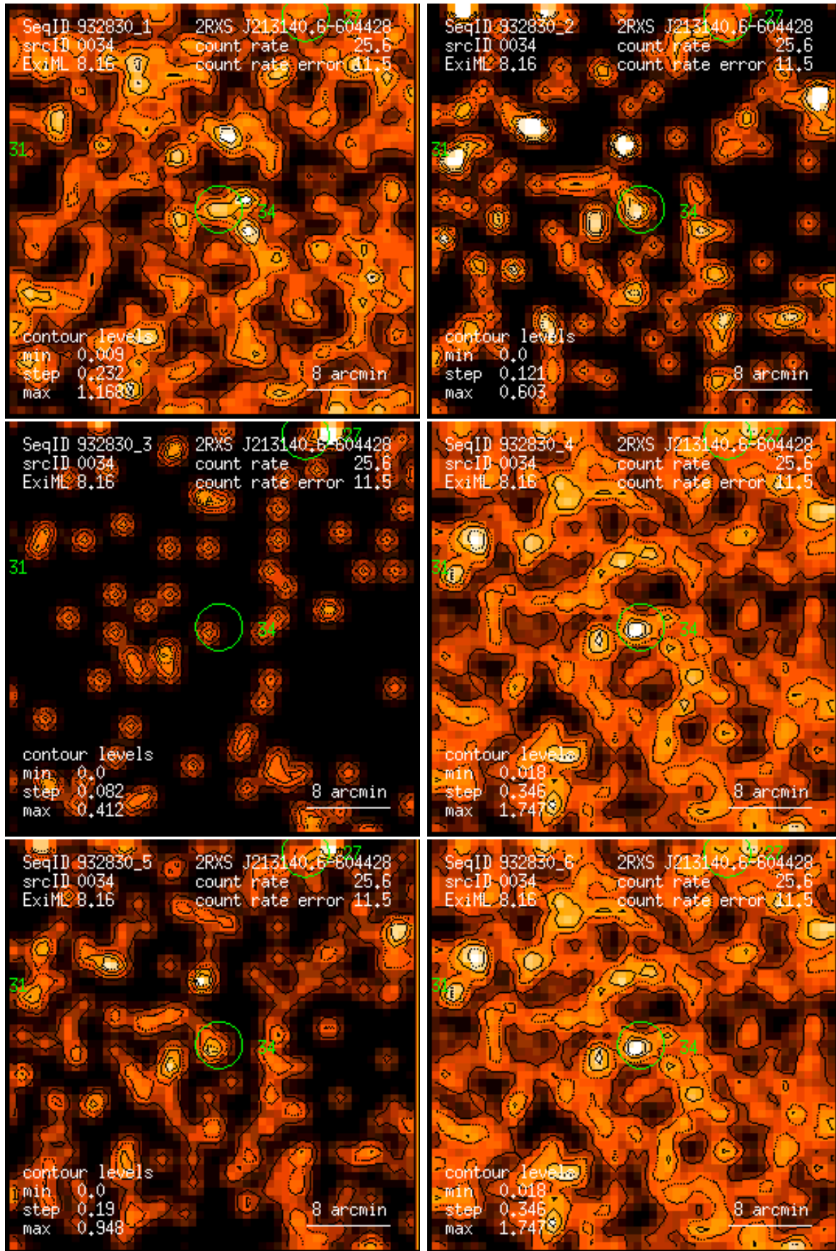
Figure 34: RASS 932830: detection 0034: band rate images, Gaussian filter: (1) PSPC channels 11 – 41, (2) 52 – 90, (3) 91 – 201, (4) 11 – 235, (5) 52 – 201, (6) 11 – 201. Broad band rates in counts/ks. Band rate contour levels in counts/ks/arcmin 2 .
