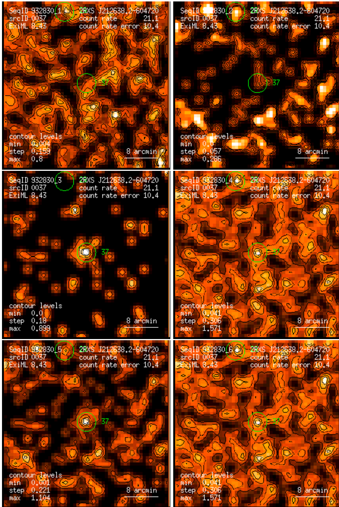
Figure 37: RASS 932830: detection 0037: band rate images, Gaussian filter: (1) PSPC channels 11 – 41, (2) 52 – 90, (3) 91 – 201, (4) 11 – 235, (5) 52 – 201, (6) 11 – 201. Broad band rates in counts/ks. Band rate contour levels in counts/ks/arcmin 2 .
