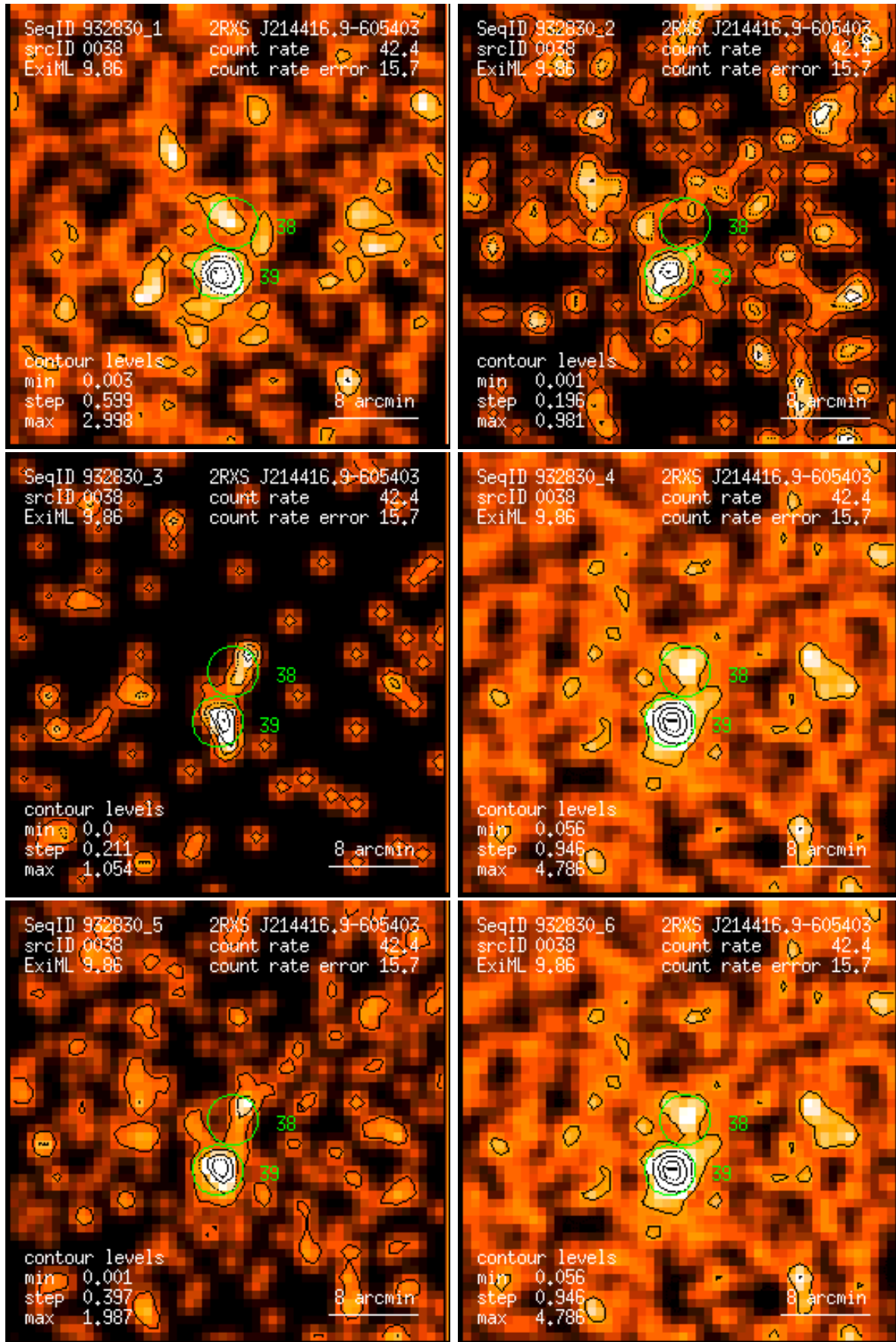
Figure 38: RASS 932830: detection 0038: band rate images, Gaussian filter: (1) PSPC channels 11 – 41, (2) 52 – 90, (3) 91 – 201, (4) 11 – 235, (5) 52 – 201, (6) 11 – 201. Broad band rates in counts/ks. Band rate contour levels in counts/ks/arcmin 2 .
