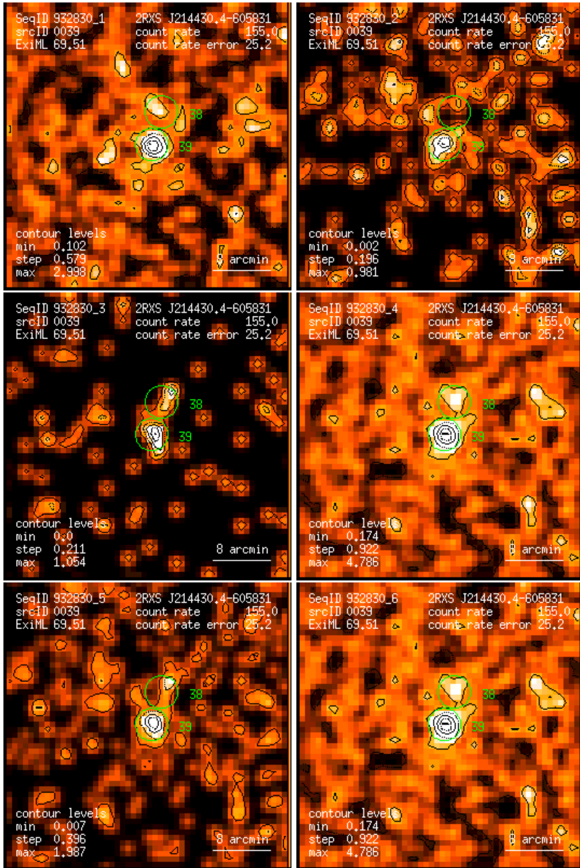
Figure 39: RASS 932830: detection 0039: band rate images, Gaussian filter: (1) PSPC channels 11 – 41, (2) 52 – 90, (3) 91 – 201, (4) 11 – 235, (5) 52 – 201, (6) 11 – 201. Broad band rates in counts/ks. Band rate contour levels in counts/ks/arcmin 2 .
