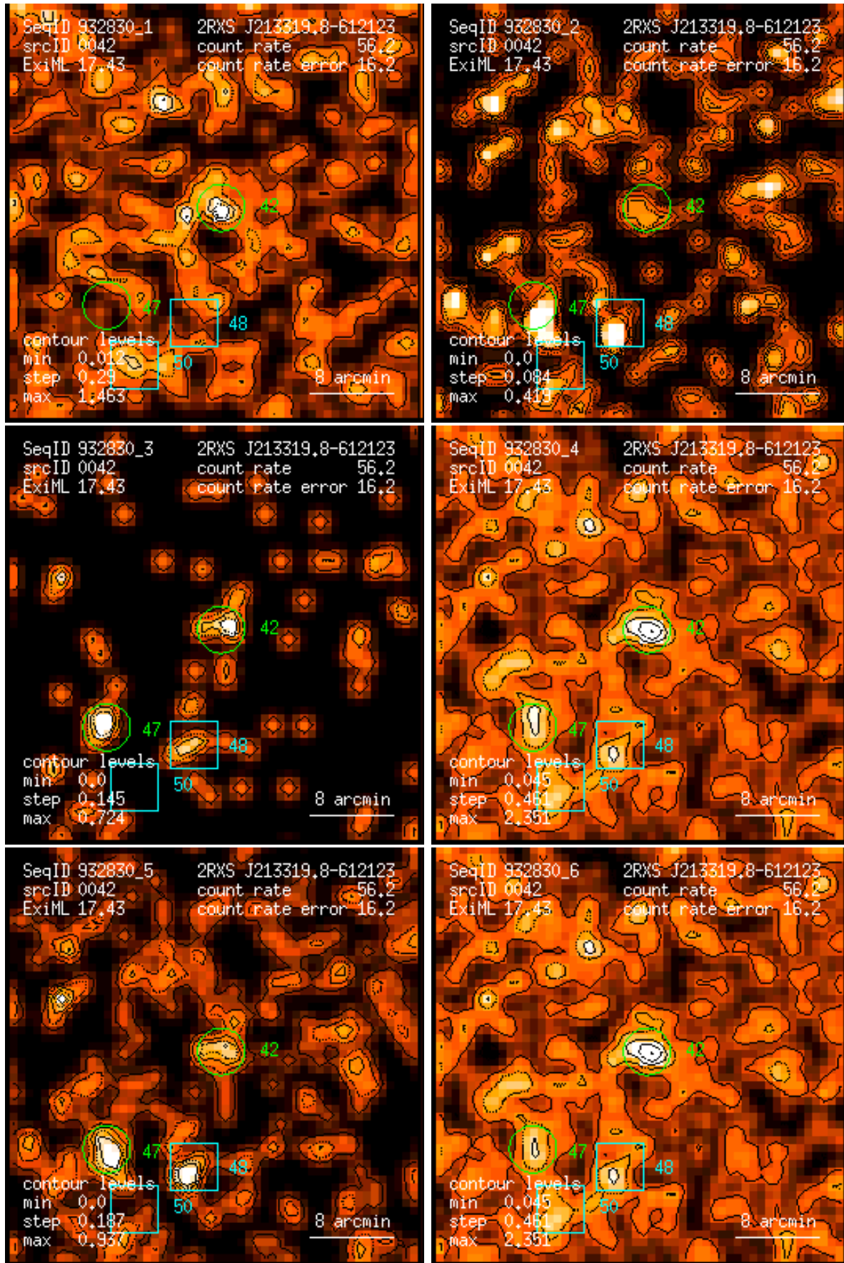
Figure 42: RASS 932830: detection 0042: band rate images, Gaussian filter: (1) PSPC channels 11 – 41, (2) 52 – 90, (3) 91 – 201, (4) 11 – 235, (5) 52 – 201, (6) 11 – 201. Broad band rates in counts/ks. Band rate contour levels in counts/ks/arcmin 2 .
