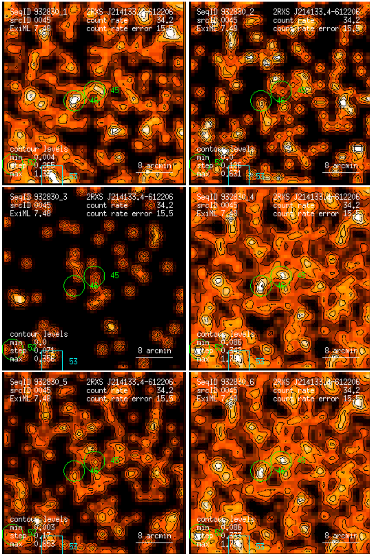
Figure 45: RASS 932830: detection 0045: band rate images, Gaussian filter: (1) PSPC channels 11 – 41, (2) 52 – 90, (3) 91 – 201, (4) 11 – 235, (5) 52 – 201, (6) 11 – 201. Broad band rates in counts/ks. Band rate contour levels in counts/ks/arcmin 2 .
