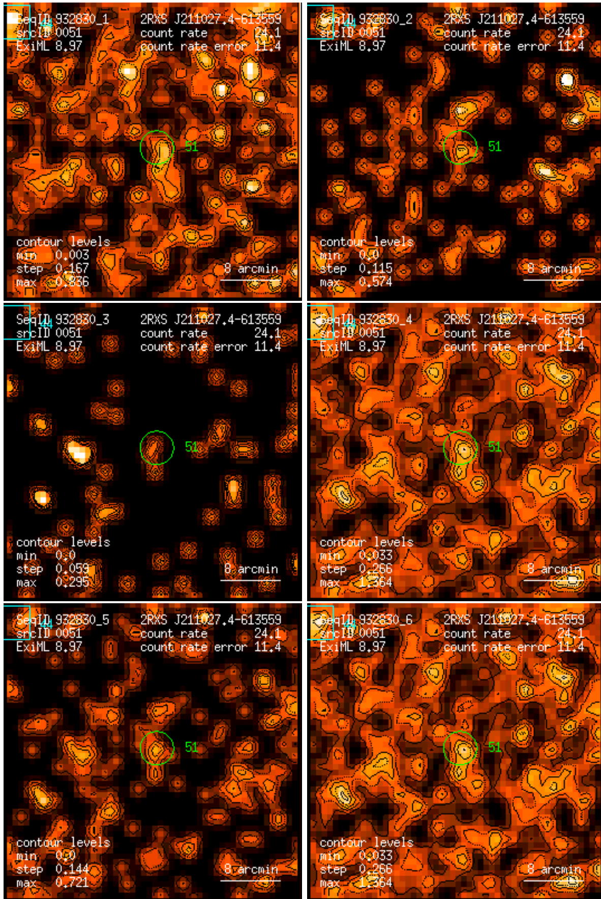
Figure 51: RASS 932830: detection 0051: band rate images, Gaussian filter: (1) PSPC channels 11 – 41, (2) 52 – 90, (3) 91 – 201, (4) 11 – 235, (5) 52 – 201, (6) 11 – 201. Broad band rates in counts/ks. Band rate contour levels in counts/ks/arcmin 2 .
