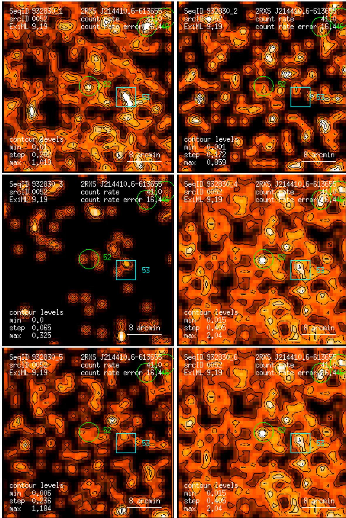
Figure 52: RASS 932830: detection 0052: band rate images, Gaussian filter: (1) PSPC channels 11 – 41, (2) 52 – 90, (3) 91 – 201, (4) 11 – 235, (5) 52 – 201, (6) 11 – 201. Broad band rates in counts/ks. Band rate contour levels in counts/ks/arcmin 2 .
