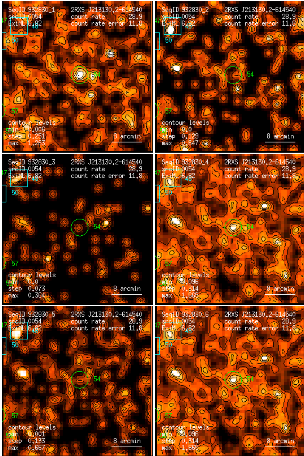
Figure 54: RASS 932830: detection 0054: band rate images, Gaussian filter: (1) PSPC channels 11 – 41, (2) 52 – 90, (3) 91 – 201, (4) 11 – 235, (5) 52 – 201, (6) 11 – 201. Broad band rates in counts/ks. Band rate contour levels in counts/ks/arcmin 2 .
