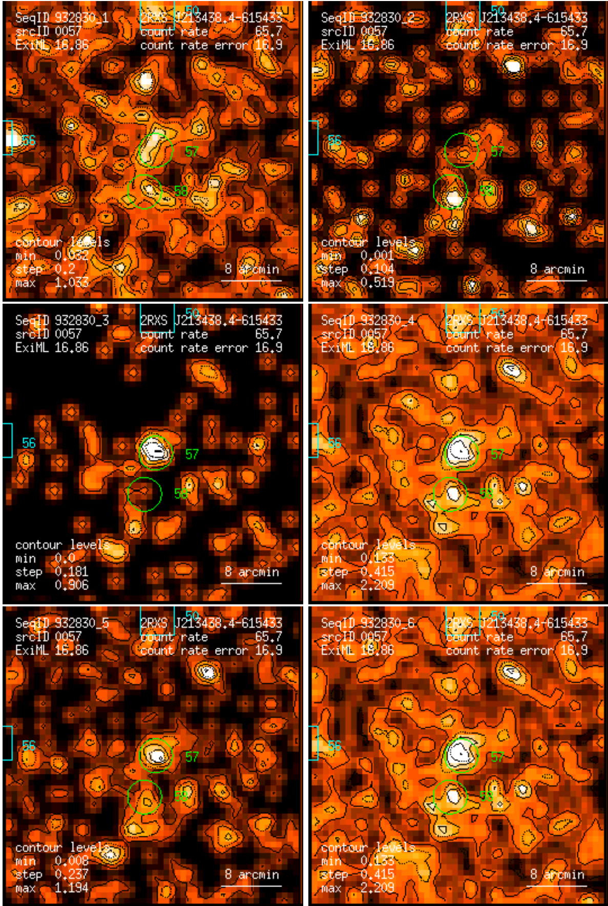
Figure 57: RASS 932830: detection 0057: band rate images, Gaussian filter: (1) PSPC channels 11 – 41, (2) 52 – 90, (3) 91 – 201, (4) 11 – 235, (5) 52 – 201, (6) 11 – 201. Broad band rates in counts/ks. Band rate contour levels in counts/ks/arcmin 2 .
