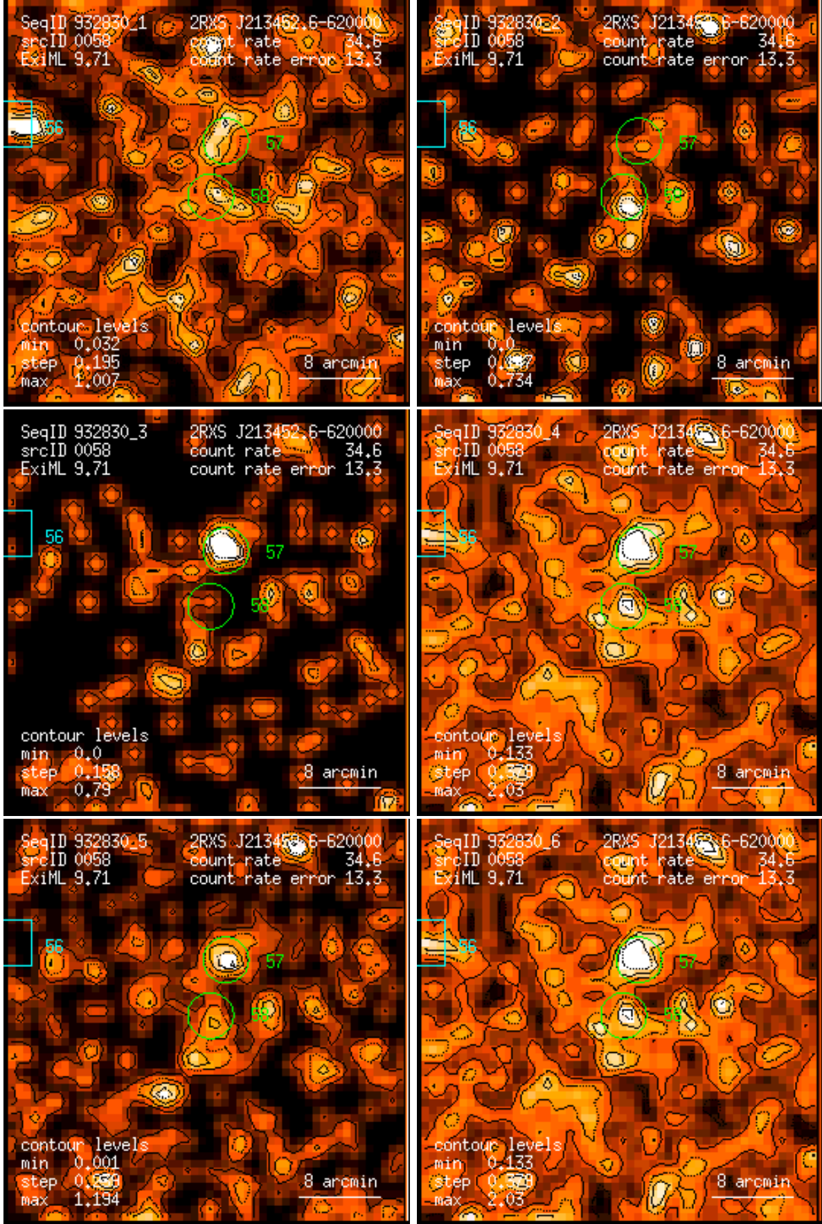
Figure 58: RASS 932830: detection 0058: band rate images, Gaussian filter: (1) PSPC channels 11 – 41, (2) 52 – 90, (3) 91 – 201, (4) 11 – 235, (5) 52 – 201, (6) 11 – 201. Broad band rates in counts/ks. Band rate contour levels in counts/ks/arcmin 2 .
