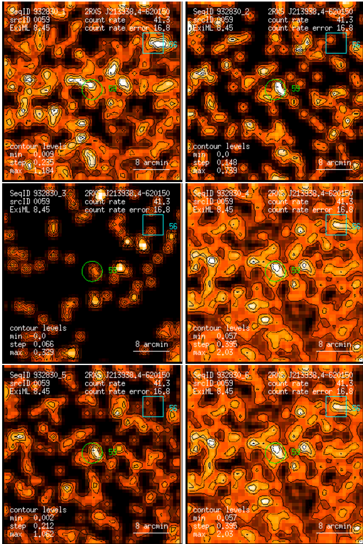
Figure 59: RASS 932830: detection 0059: band rate images, Gaussian filter: (1) PSPC channels 11 – 41, (2) 52 – 90, (3) 91 – 201, (4) 11 – 235, (5) 52 – 201, (6) 11 – 201. Broad band rates in counts/ks. Band rate contour levels in counts/ks/arcmin 2 .
