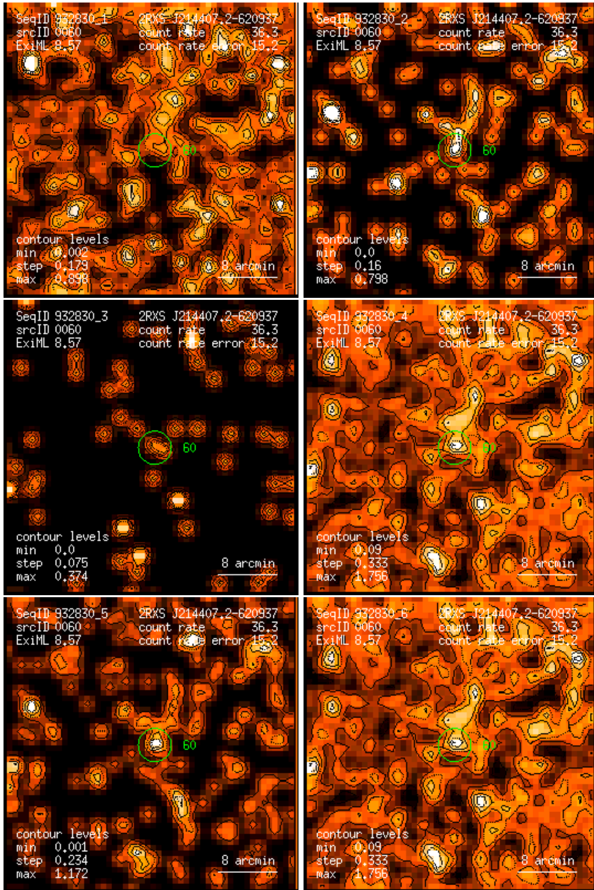
Figure 60: RASS 932830: detection 0060: band rate images, Gaussian filter: (1) PSPC channels 11 – 41, (2) 52 – 90, (3) 91 – 201, (4) 11 – 235, (5) 52 – 201, (6) 11 – 201. Broad band rates in counts/ks. Band rate contour levels in counts/ks/arcmin 2 .
