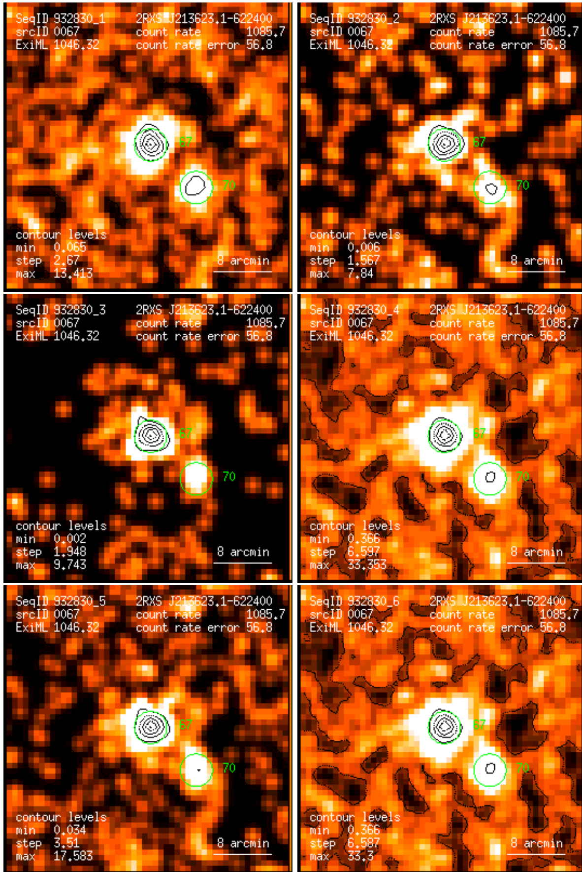
Figure 67: RASS 932830: detection 0067: band rate images, Gaussian filter: (1) PSPC channels 11 – 41, (2) 52 – 90, (3) 91 – 201, (4) 11 – 235, (5) 52 – 201, (6) 11 – 201. Broad band rates in counts/ks. Band rate contour levels in counts/ks/arcmin 2 .
