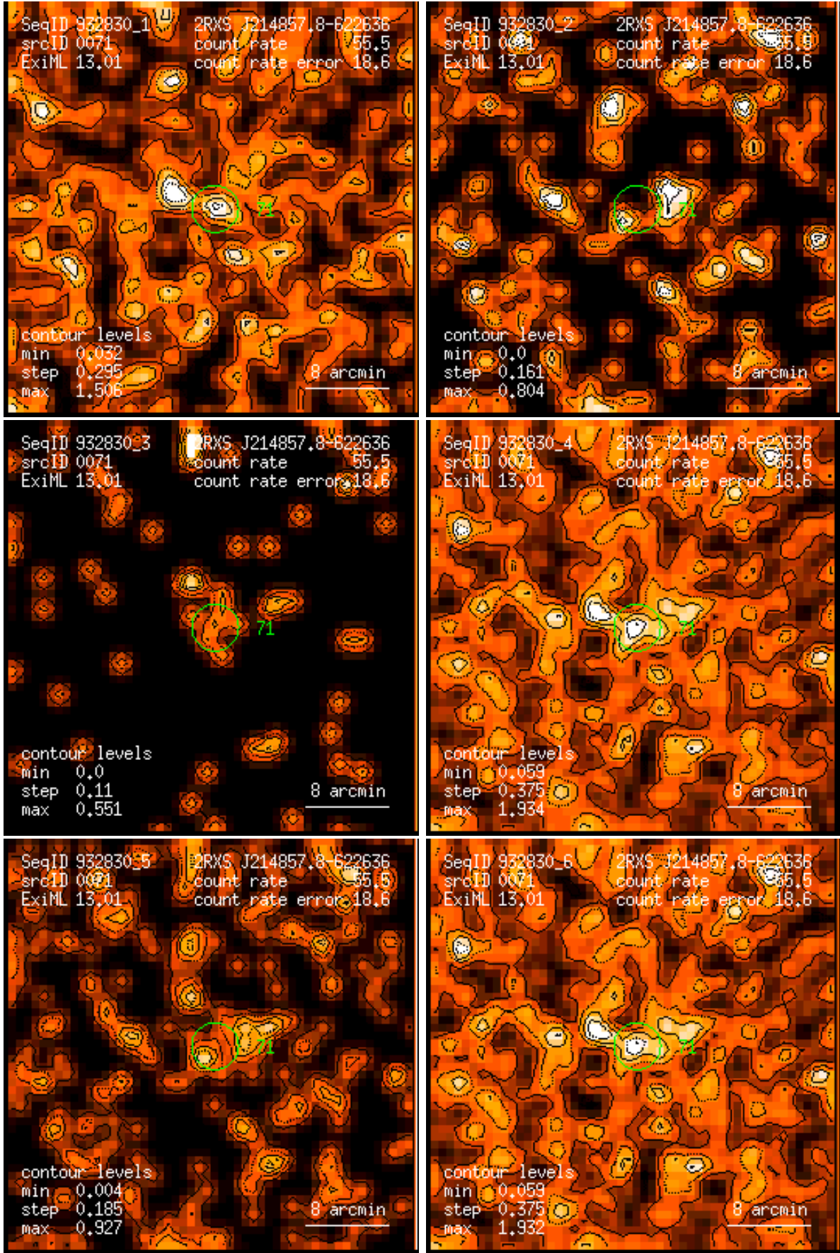
Figure 71: RASS 932830: detection 0071: band rate images, Gaussian filter: (1) PSPC channels 11 – 41, (2) 52 – 90, (3) 91 – 201, (4) 11 – 235, (5) 52 – 201, (6) 11 – 201. Broad band rates in counts/ks. Band rate contour levels in counts/ks/arcmin 2 .
