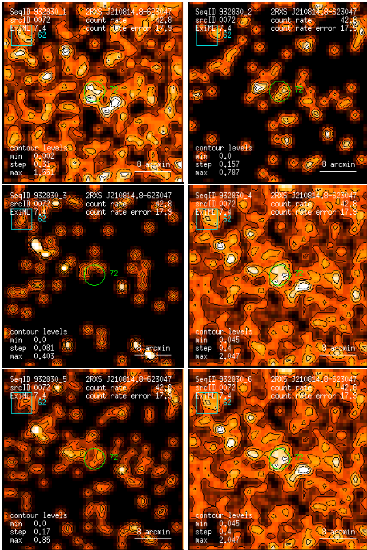
Figure 72: RASS 932830: detection 0072: band rate images, Gaussian filter: (1) PSPC channels 11 – 41, (2) 52 – 90, (3) 91 – 201, (4) 11 – 235, (5) 52 – 201, (6) 11 – 201. Broad band rates in counts/ks. Band rate contour levels in counts/ks/arcmin 2 .
