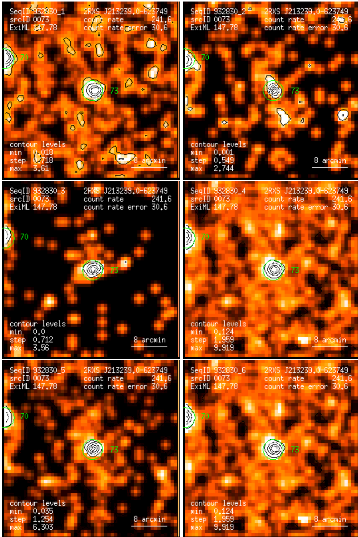
Figure 73: RASS 932830: detection 0073: band rate images, Gaussian filter: (1) PSPC channels 11 – 41, (2) 52 – 90, (3) 91 – 201, (4) 11 – 235, (5) 52 – 201, (6) 11 – 201. Broad band rates in counts/ks. Band rate contour levels in counts/ks/arcmin 2 .
