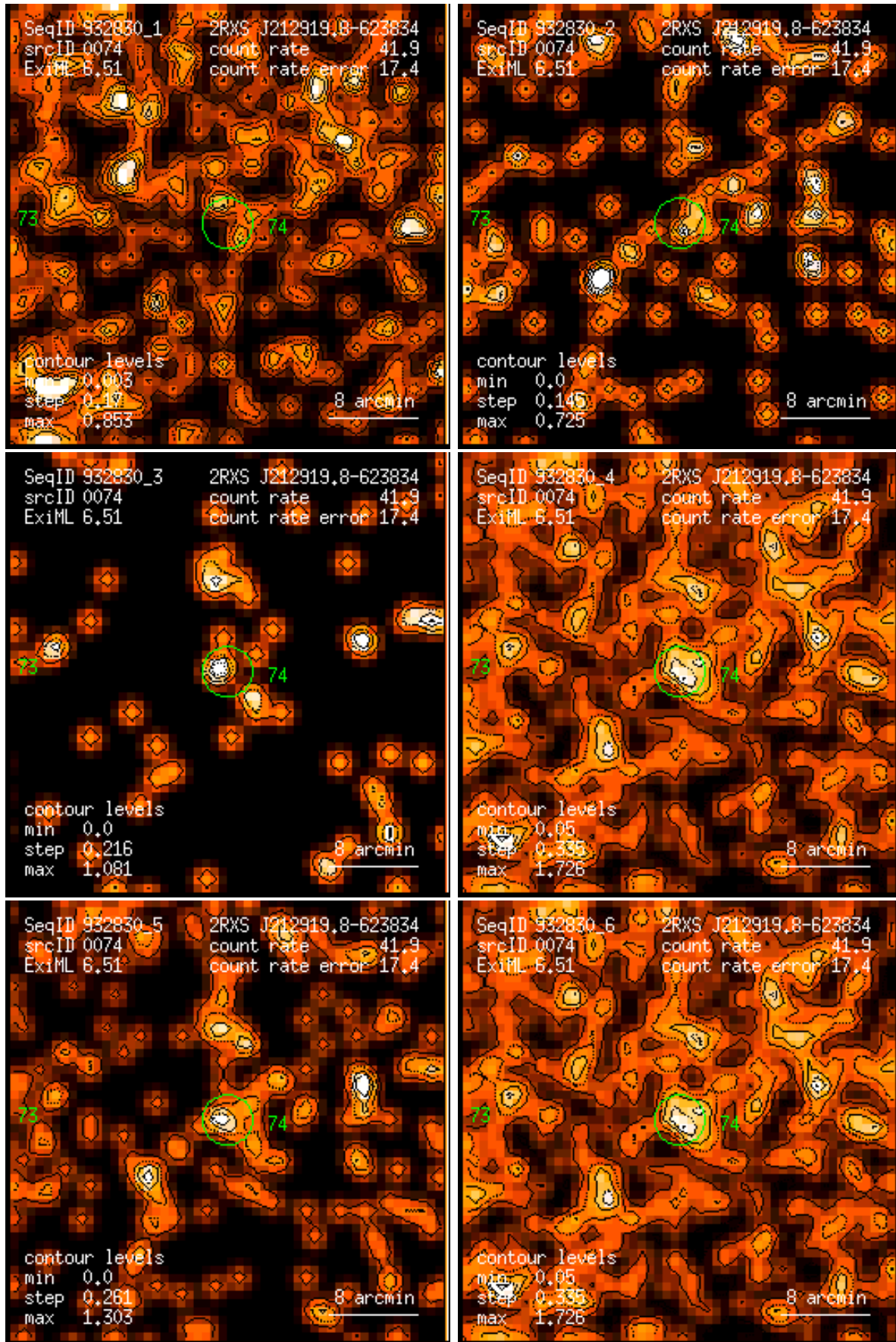
Figure 74: RASS 932830: detection 0074: band rate images, Gaussian filter: (1) PSPC channels 11 – 41, (2) 52 – 90, (3) 91 – 201, (4) 11 – 235, (5) 52 – 201, (6) 11 – 201. Broad band rates in counts/ks. Band rate contour levels in counts/ks/arcmin 2 .
