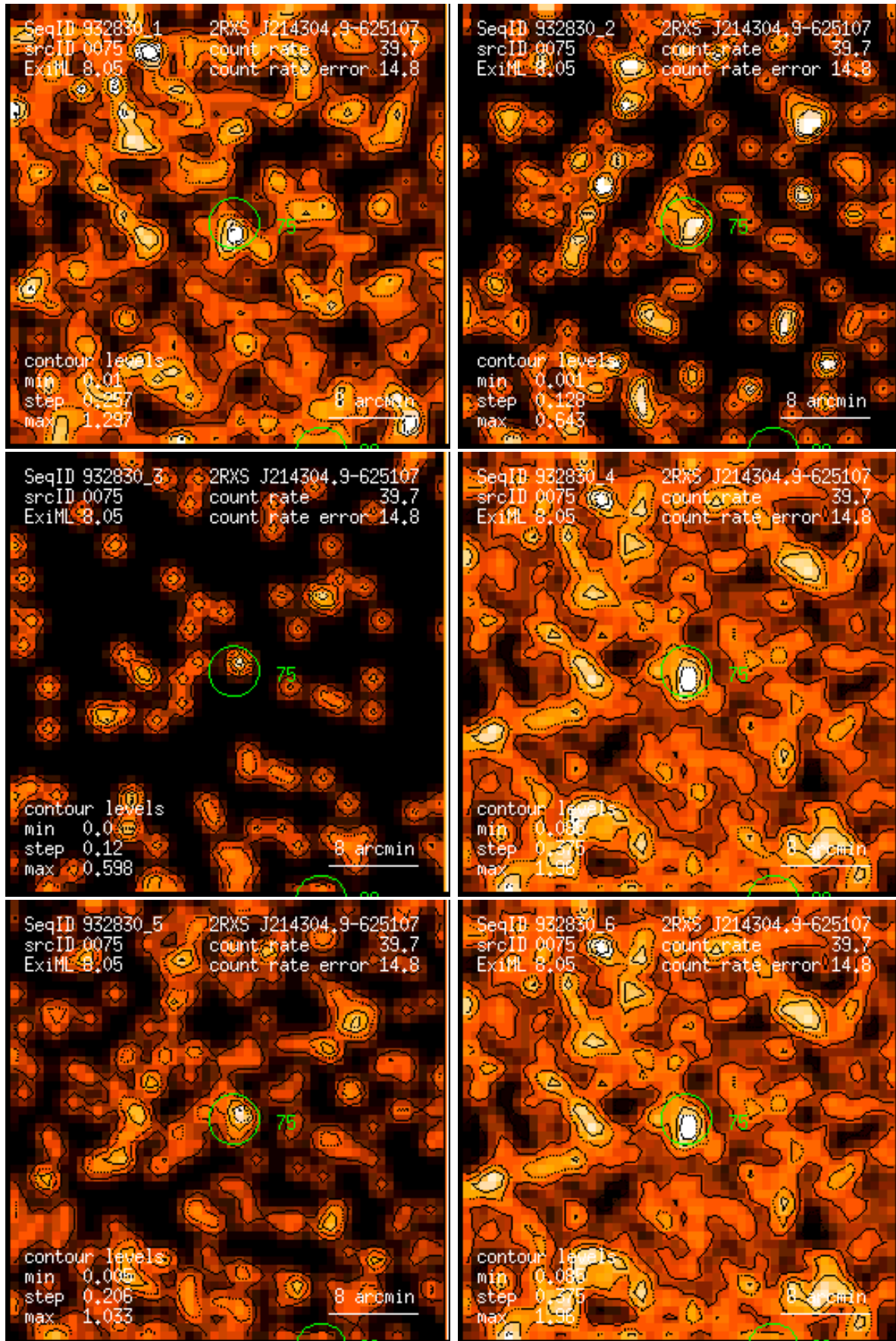
Figure 75: RASS 932830: detection 0075: band rate images, Gaussian filter: (1) PSPC channels 11 – 41, (2) 52 – 90, (3) 91 – 201, (4) 11 – 235, (5) 52 – 201, (6) 11 – 201. Broad band rates in counts/ks. Band rate contour levels in counts/ks/arcmin 2 .
