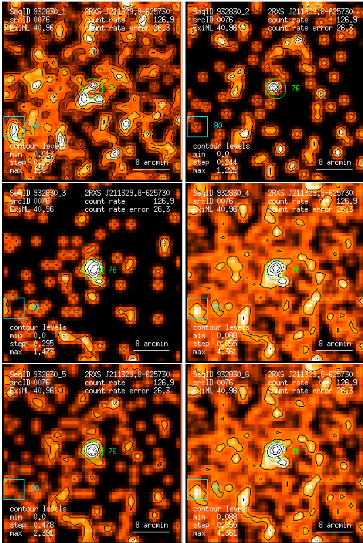
Figure 76: RASS 932830: detection 0076: band rate images, Gaussian filter: (1) PSPC channels 11 – 41, (2) 52 – 90, (3) 91 – 201, (4) 11 – 235, (5) 52 – 201, (6) 11 – 201. Broad band rates in counts/ks. Band rate contour levels in counts/ks/arcmin 2 .
