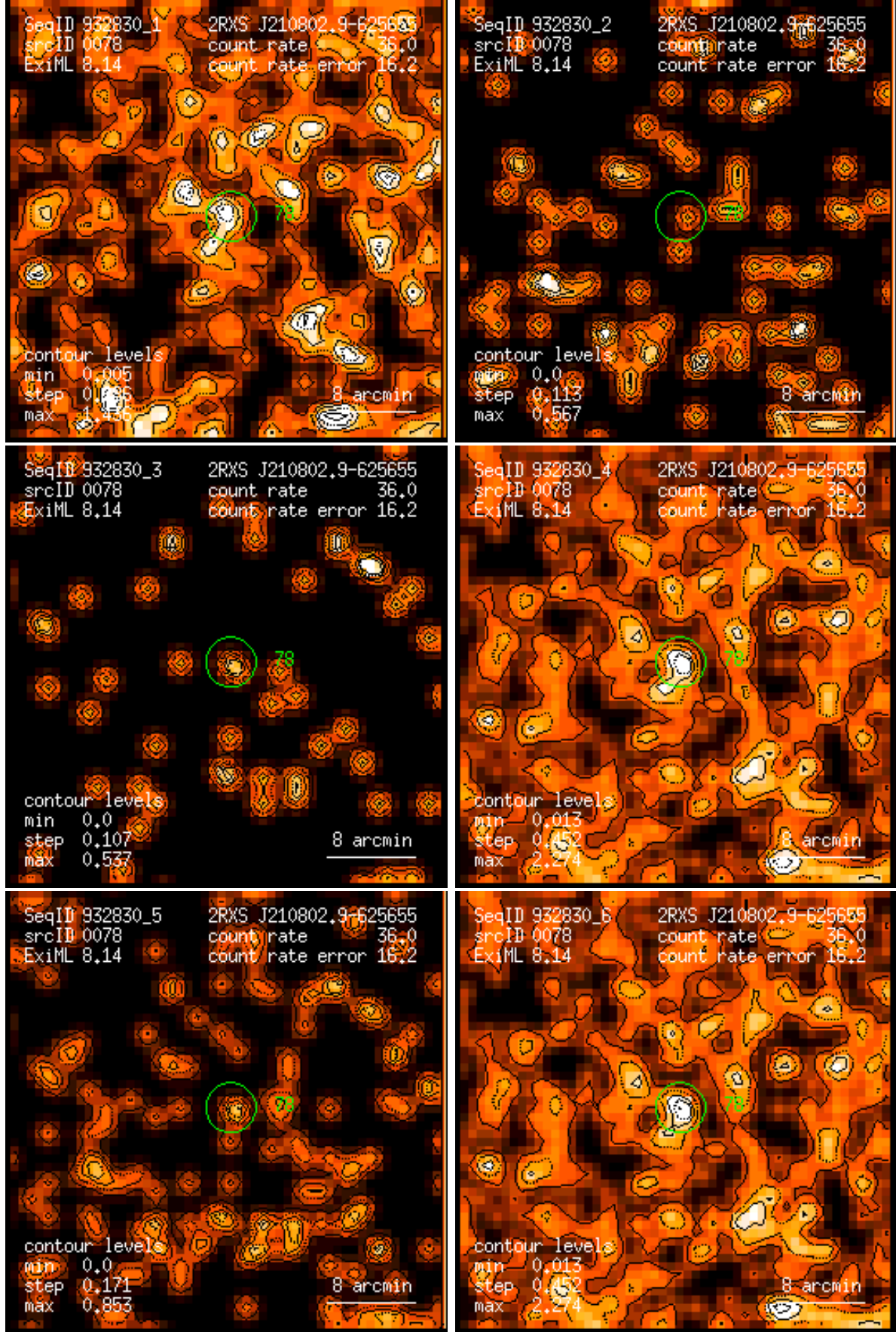
Figure 78: RASS 932830: detection 0078: band rate images, Gaussian filter: (1) PSPC channels 11 – 41, (2) 52 – 90, (3) 91 – 201, (4) 11 – 235, (5) 52 – 201, (6) 11 – 201. Broad band rates in counts/ks. Band rate contour levels in counts/ks/arcmin 2 .
