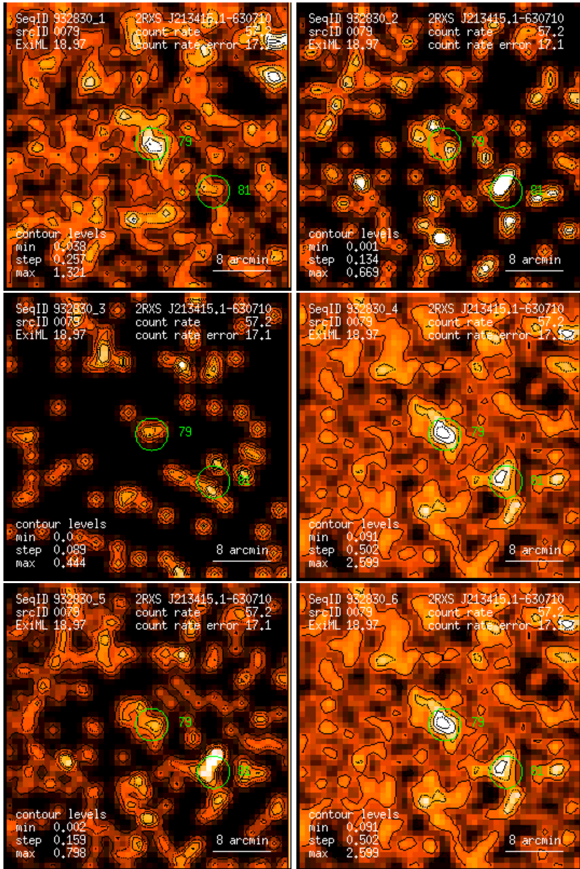
Figure 79: RASS 932830: detection 0079: band rate images, Gaussian filter: (1) PSPC channels 11 – 41, (2) 52 – 90, (3) 91 – 201, (4) 11 – 235, (5) 52 – 201, (6) 11 – 201. Broad band rates in counts/ks. Band rate contour levels in counts/ks/arcmin 2 .
