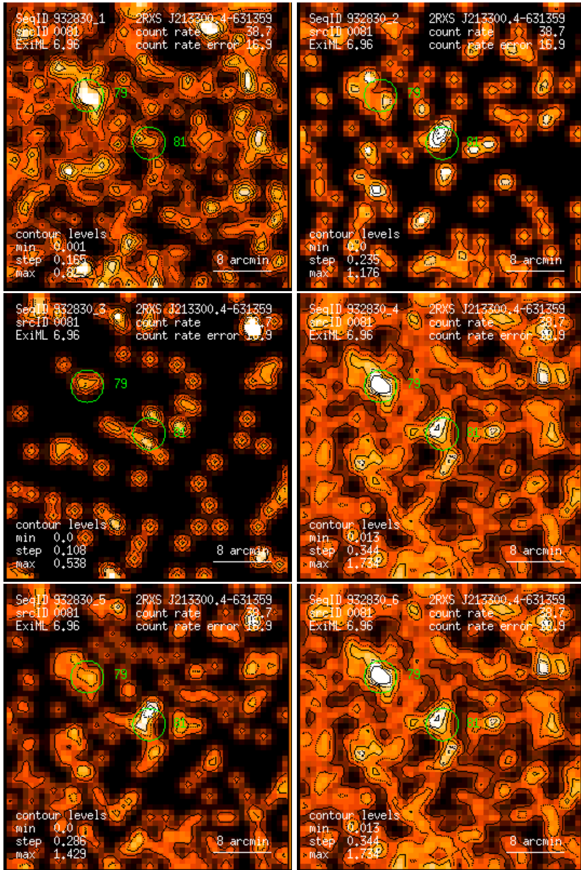
Figure 81: RASS 932830: detection 0081: band rate images, Gaussian filter: (1) PSPC channels 11 – 41, (2) 52 – 90, (3) 91 – 201, (4) 11 – 235, (5) 52 – 201, (6) 11 – 201. Broad band rates in counts/ks. Band rate contour levels in counts/ks/arcmin 2 .
