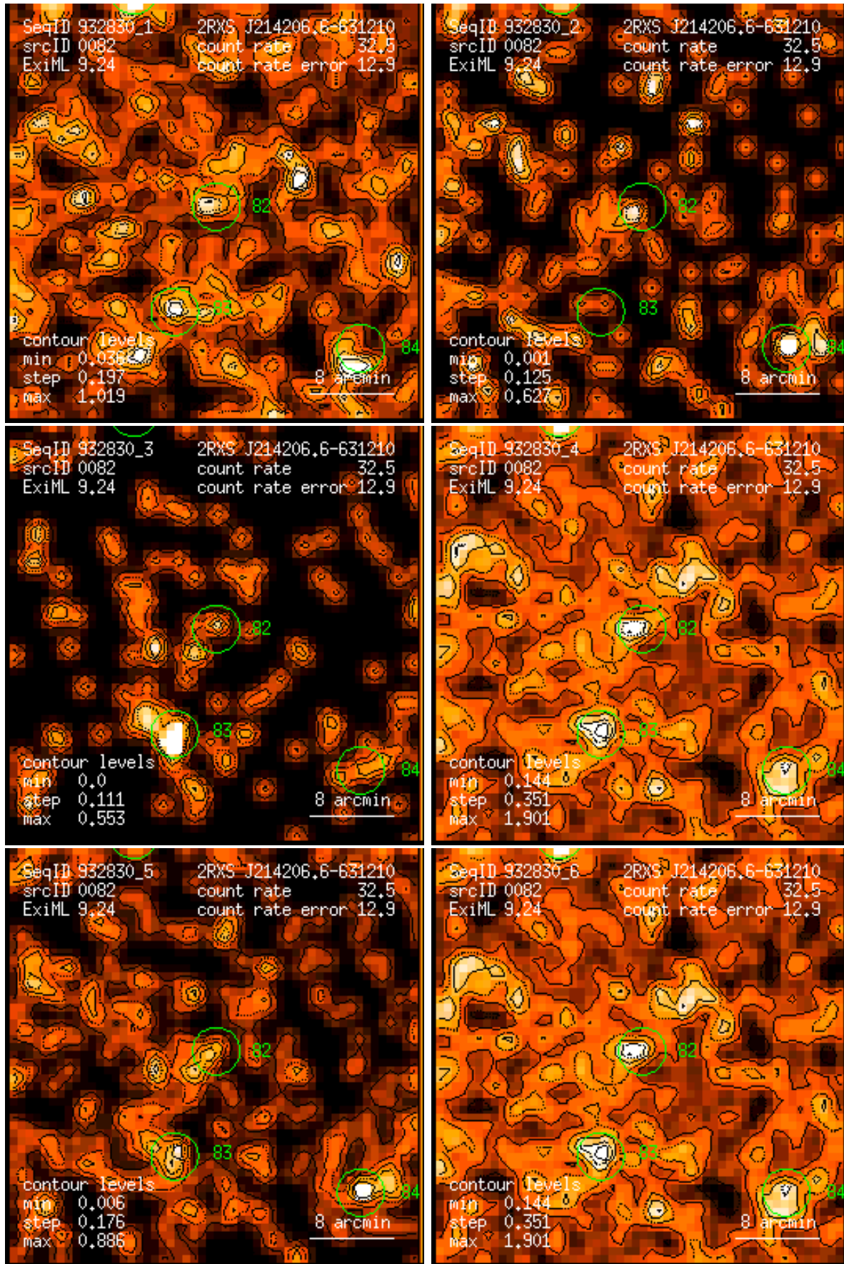
Figure 82: RASS 932830: detection 0082: band rate images, Gaussian filter: (1) PSPC channels 11 – 41, (2) 52 – 90, (3) 91 – 201, (4) 11 – 235, (5) 52 – 201, (6) 11 – 201. Broad band rates in counts/ks. Band rate contour levels in counts/ks/arcmin 2 .
